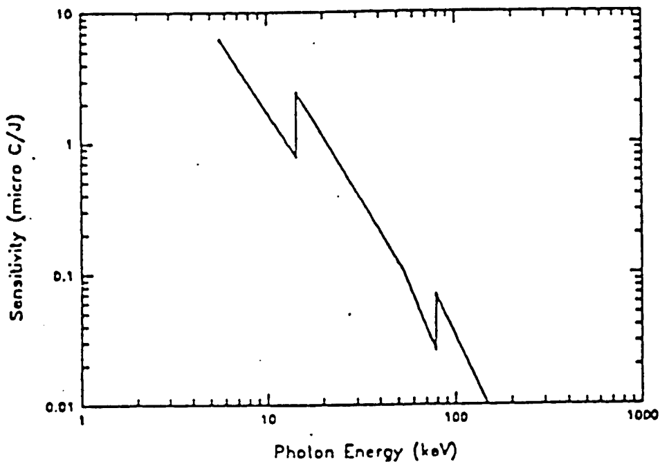
Fig 2. Sensitivity Curve
