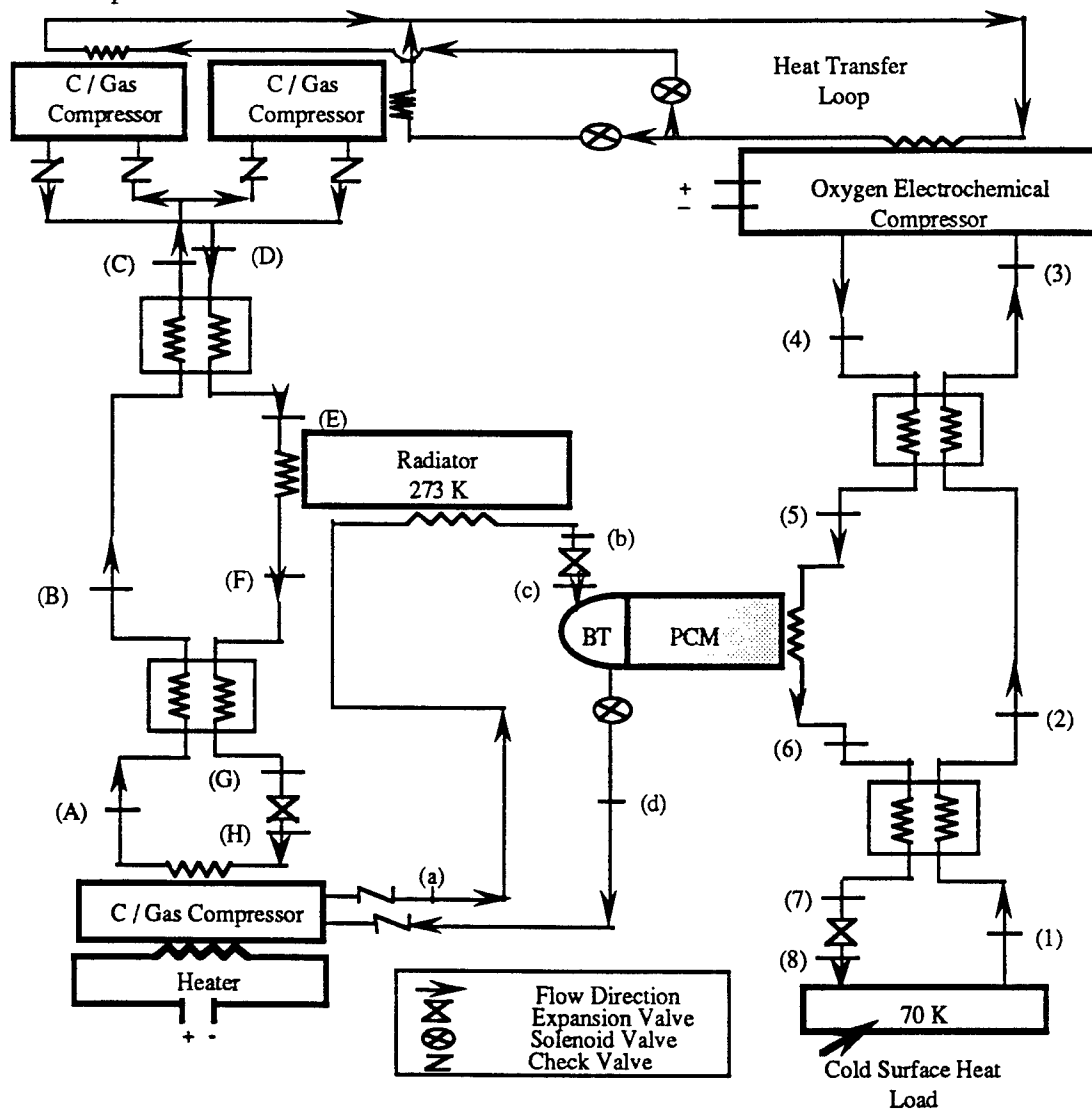
Fig. 1. Three Stage Cascade Cryocooler
