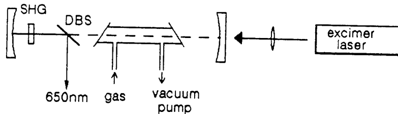
Figure 2: Experimental configuration for an excimer-laser pumped iodine laser
