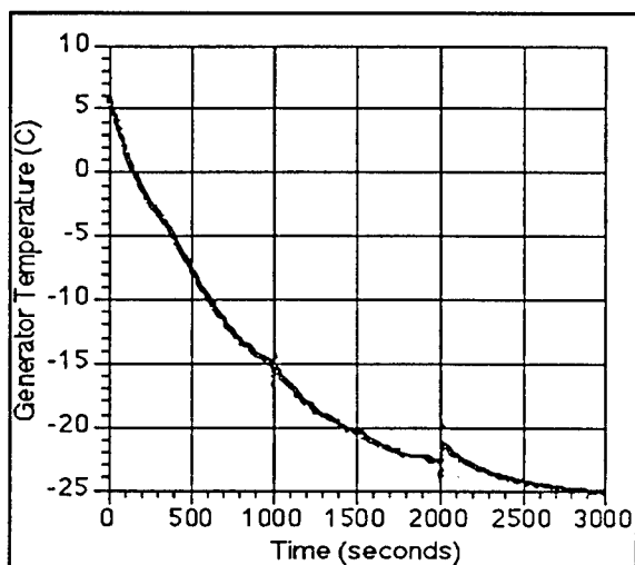
Figure (6b) RADICL Generator Temperature Profile with Respect to Time.
