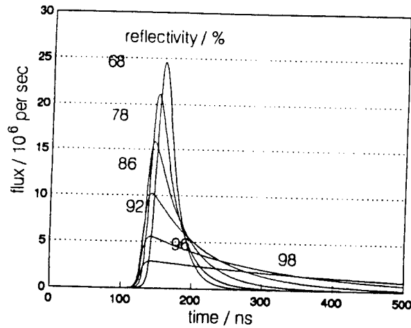
Figure 3: Calculated output power (fundamental radiation) of a gain-switched iodine laser for various reflection coefficients of the outcoupling mirror. The pump pulse duration was 20ns.
