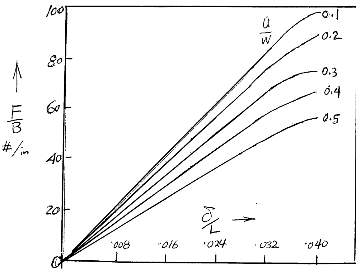
FIGURE 6 J-INTEGRAL AND LOAD VS. DISPLACEMENT FOR 2" SPECIMEN
