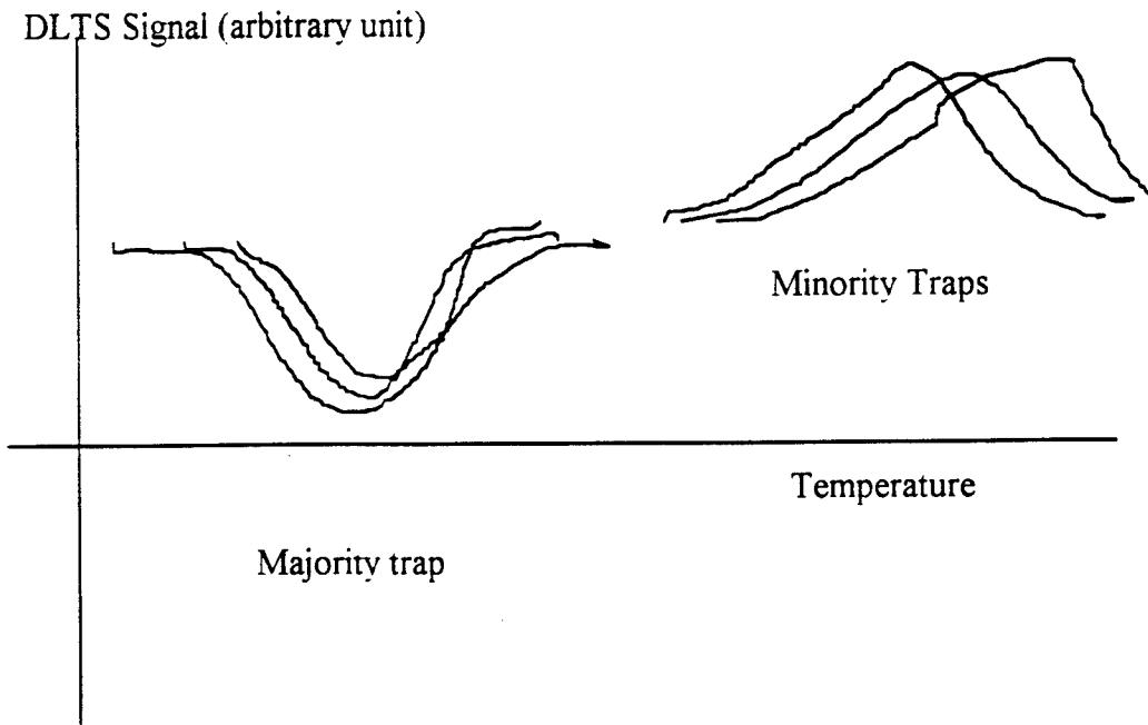
Fig.3 Typical extrema obtained during DLTS.
