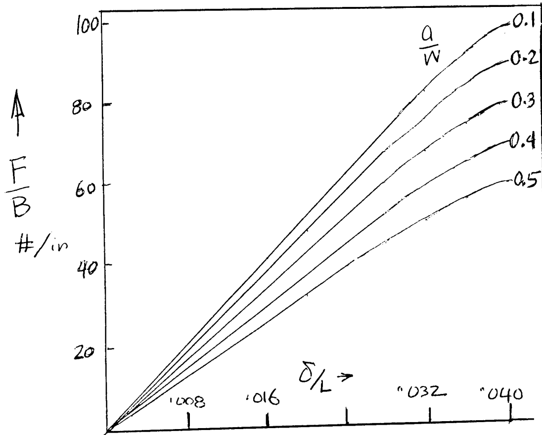
FIGURE 7 J-INTEGRAL AND LOAD VS. DISPLACEMENT FOR 3" SPECIMEN
