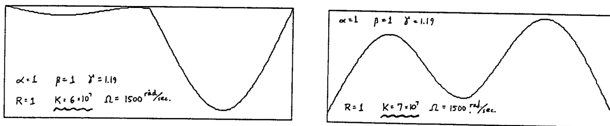
Figure 8. Response shapes for the idealized beam in reference 10 for two values of nonlinear stiffness, K.
