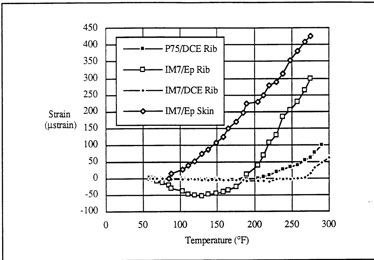
Fig. 10. Results of thermal expansion tests conducted at Aerospace Corporation.
