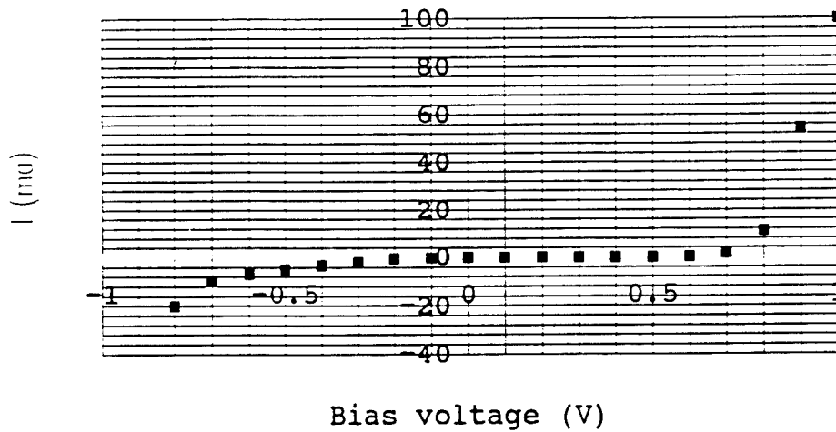
Fig. 7 I-V Characteristic of the 125x125um 2 HgCdTe diode.
