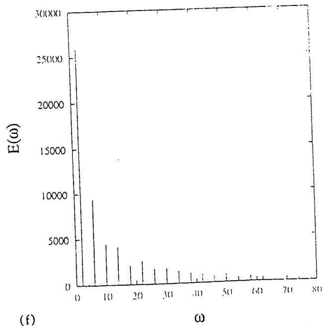
Fig. 5. Wave fields of ELF/VLF emissions (a), (c), (e) and their Fourier spectra (b), (d), (f) respond to the successive modulations of Fig. 1.
