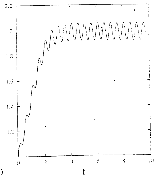
Fig. 3. Electron temperature modulation induced by two o-mode HF heaters beat for three frequency differences (a) 10 Hz, (c) 100 Hz and (e) 1000 Hz; (b), (d) and (f) are the Fourier spectra of (a), (c) and (e) respectively.
