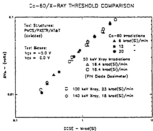
Fig 4. Overlay of PMOS Threshold Sensitivity Data
