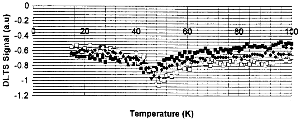
Fig. 14 DLTS signal for trap T_{E1}
