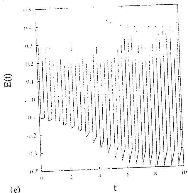
Fig. 5. Wave fields of ELF/VLF emissions (a), (c), (e) and their Fourier spectra (b), (d), (f) respond to the successive modulations of Fig. 1.
