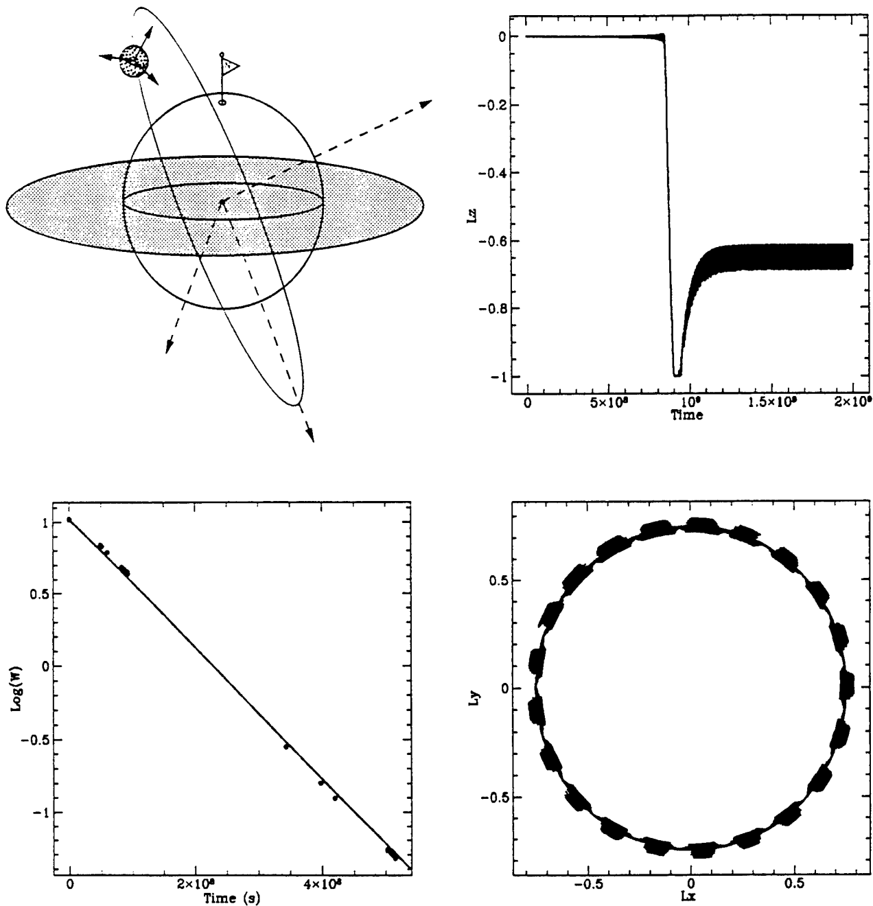
Fig. 2: The spin dynamics of LAGEOS: Numerical Results: We present here results from our numerical simulation of the dynamic evolution of the LAGEOS satellite (top left figure). The evolution of the satellite's angular momentum reveals three unique phases as demonstrated in the plot of the component of angular momentum orthogonal to the orbital plane (top right). The first phase is characterized by an exponential decrease in spin of the satellite with negligible nutation and precession. In the first phase, the decay in spin for a 17 cm radius sphere of brass agrees with the data (bottom left). When the angular velocity decays to a value comparable to the orbital angular velocity the nutation and precession increase and the angular momentum vector lifts off the orbital plane and settles down orthogonal to the orbital plane. The third phase is characterized by a drift of the angular momentum vector \approx 40 deg off the orbital plane. It sweeps out a cone centered on the orthogonal to the orbital plane with an opening angle of 100 deg. All characteristic angular velocities are of the order of the orbital angular velocity.
