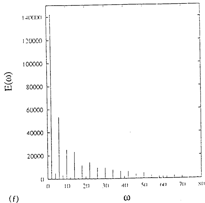
Fig. 8. Wave fields of ELF/VLF emissions (a), (c), (e) and their Fourier spectra (b), (d), (f) respond to the temperature modulations of Fig. 4.
