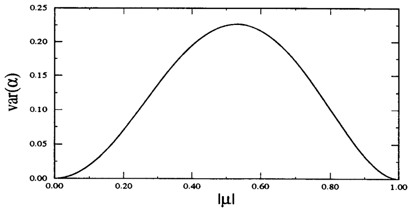
Figure 1: Cramer-Rao lower bound for the normalized variance of any unbiased estimator of \alpha when amplitude measurements are made.
