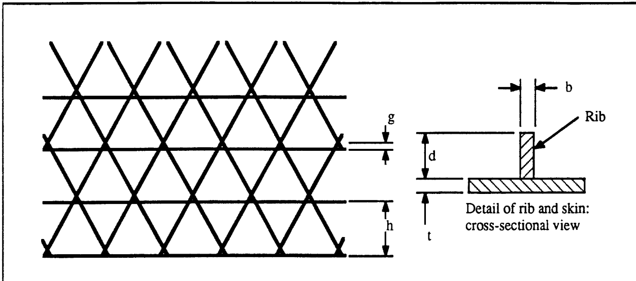
Fig. 2. Typical geometry for the flat panel isogrids studied in this work. The wide black lines are the ribs. The dimensions were: d = 0.52 in, b = .052 in, h = 3.2 in, and g = 0.3 in. The dimension t depended on the number of skin plies (see Table 1).
