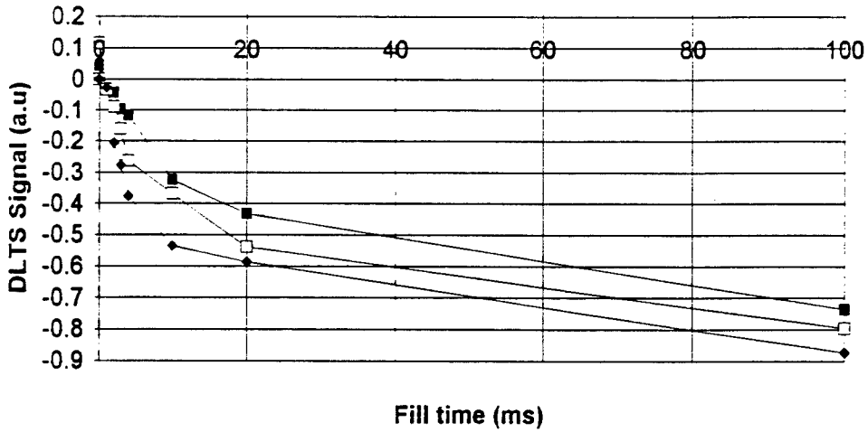
Fig. 13 DLTS signal as a function of fill time for trap T_{H2} ( V_{bias} = -.15; V_{pls} = .15 )
