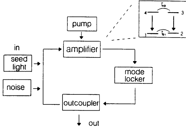
Figure 5: Block diagram of the simulation of mode beating and modelocking
