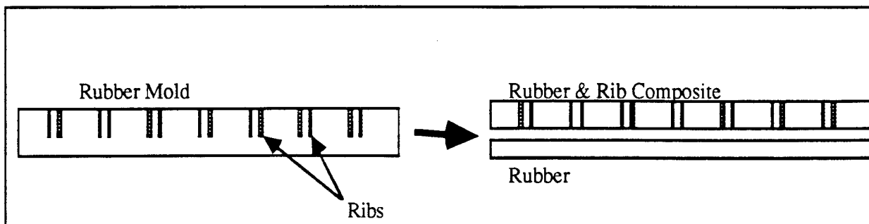
Fig. 8. Schematic showing how the rubber mold and prepreg tows (uncured ribs) were modeled by a two-layer laminate. The upper layer had the properties of a quasi-isotropic fiber-reinforced composite where the matrix was the rubber material and the fibers were the tows. The bottom layer had the properties of the rubber alone.
