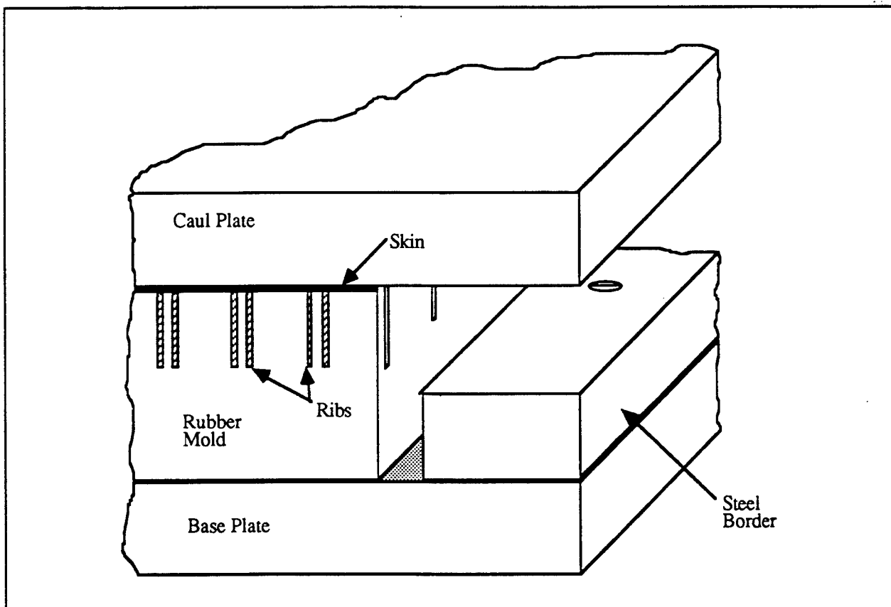
Fig. 3. Schematic diagram of basic tooling used in original manufacturing of isogrid panels. The ribs were formed by winding prepreg tow into slots in the silicone rubber mold. Prepreg tape was then laid over the ribs in the mold to form the skin. Note the 0.25 in gap between the steel borders and the rubber mold. Bagging material and release sheets are not shown.
