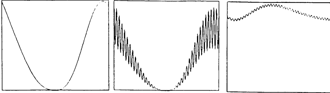
Figure 7: Laser power after gain saturation is reached for free-running (left), an amplitude-modulated (middle), and seeded (right) laser. Parameters: T_{43} = 10ns , T_{21} = 100ps , \tau_1 = \tau_2 = 100ps , p_2^2 = 2p_1^2
