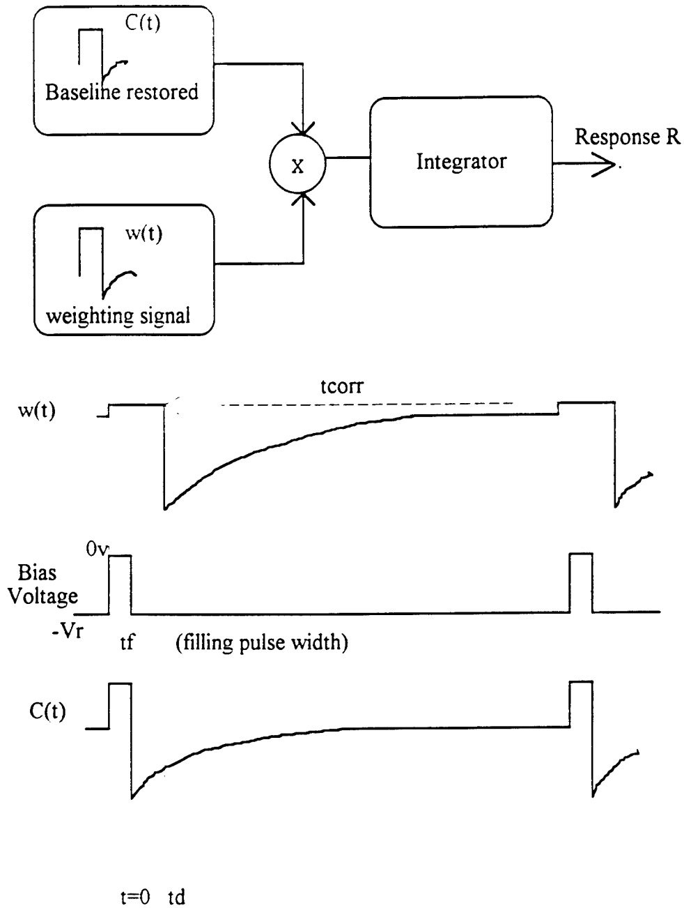
Fig. 2 Basic description of the exponential correlator. Note that the weighting signal and the bias voltage are synchronized
