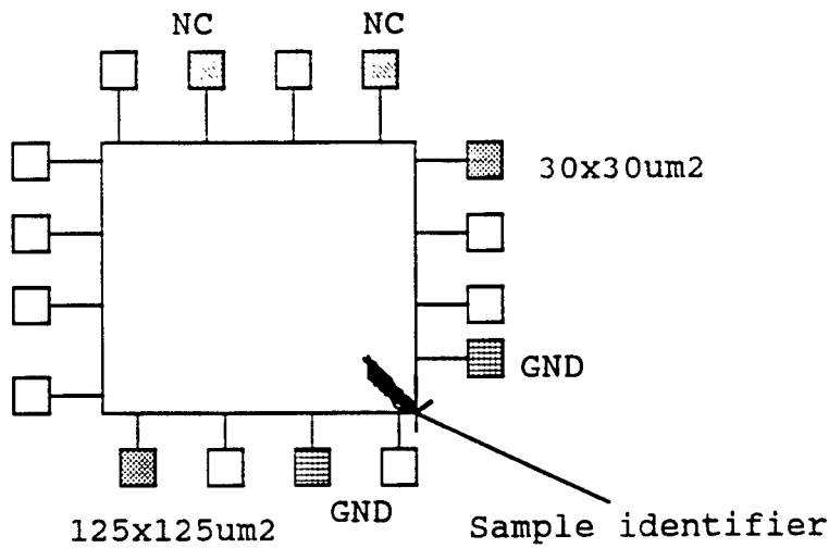
Fig. 6 \text{Hg}_{0.724}\text{Cd}_{0.276}\text{Te} samples selected for evaluation. Only the samples 125x125um 2 and 30x30um 2 had a good I-V characteristic.
