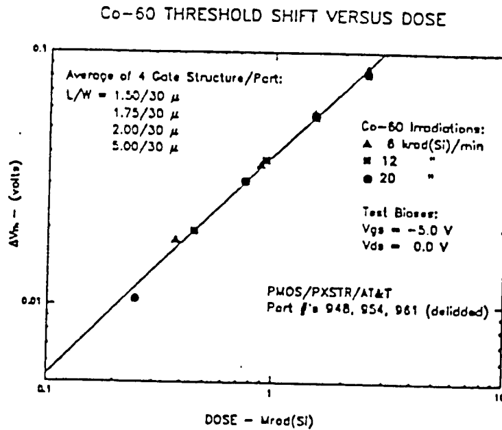
Fig 3. PMOS Threshold Sensitivity for 60 Co
