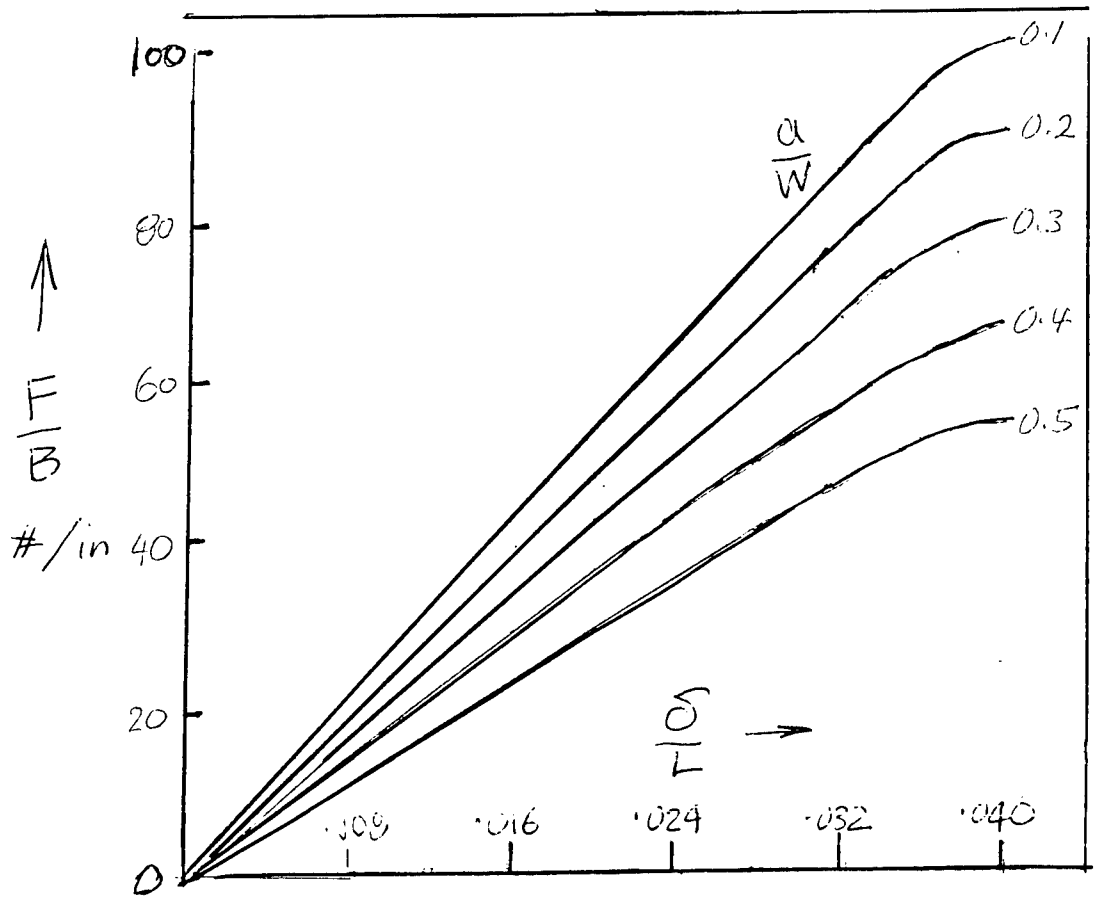
FIGURE 5 J-INTEGRAL AND LOAD VS. DISPLACEMENT FOR 1" SPECIMEN
