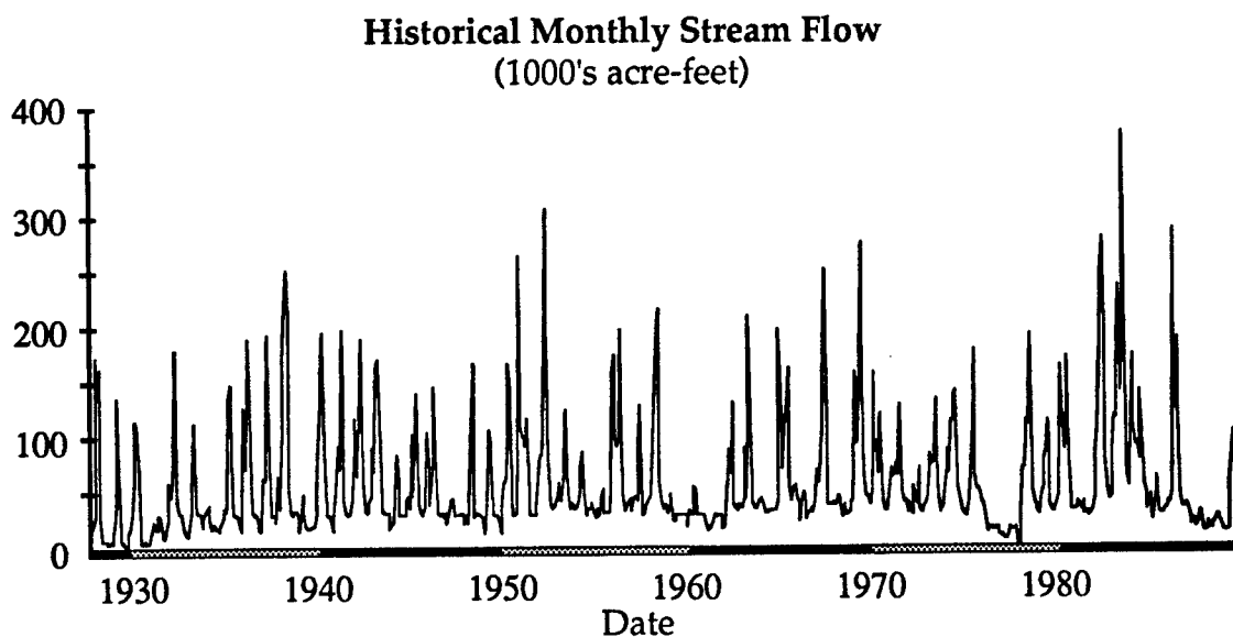
Fig. II-2. Stream-flow hydrograph of the Mokelumne River.
