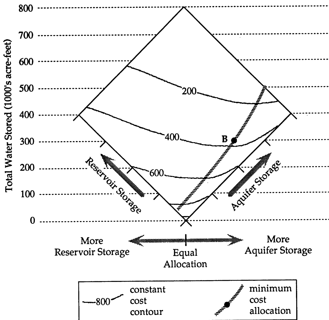
Fig. II-10. Contour plot of expected costs versus total amount and allocation of stored water. Amount of water stored in reservoir and aquifer can be measured diagonally from zero. The results are for November in the first year of a four-year planning horizon when October's stream flow was above average (60,000 acre-feet).
