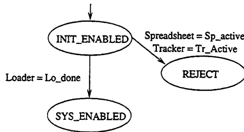
Figure 7.2: Receptive safety rules for the AEGIS system
