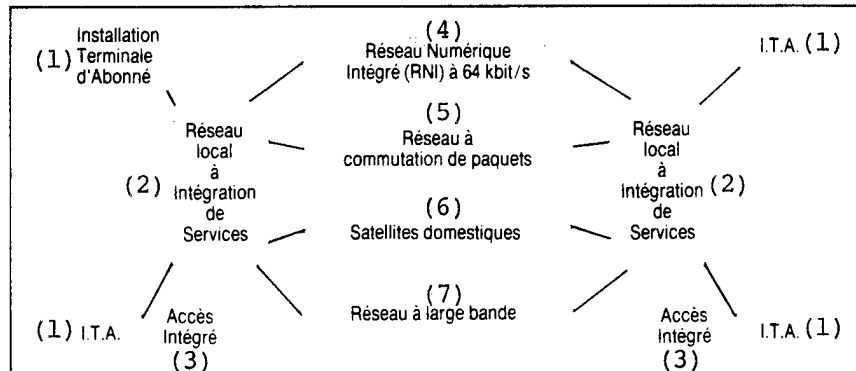
Target ISDN defined in CNET study of an integrated voice and data network.
