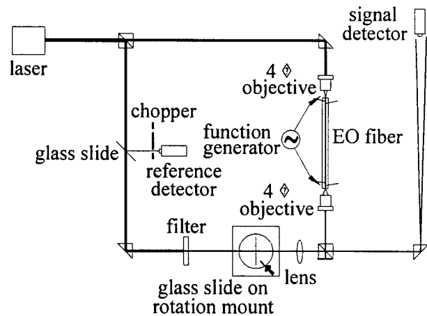
Figure 5. The electrooptic experiment.
