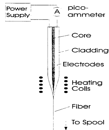
Figure 2. Drawing a fiber while poling with indium electrodes.
