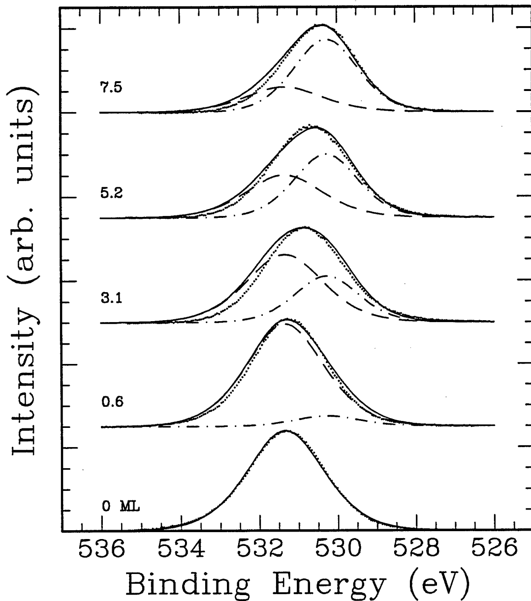
Figure 7.8. Experimental and simulated XPS O 1s peaks for a -1.07 eV total shift. The film was produced by 60°C dose and 460°C anneal cycles. The dots represent experimental peaks after background subtraction. The dash-dash, dot-dash, and solid lines represent the oxygen from O - Al bonding, O - Ti bonding, and the composite peak, respectively.
