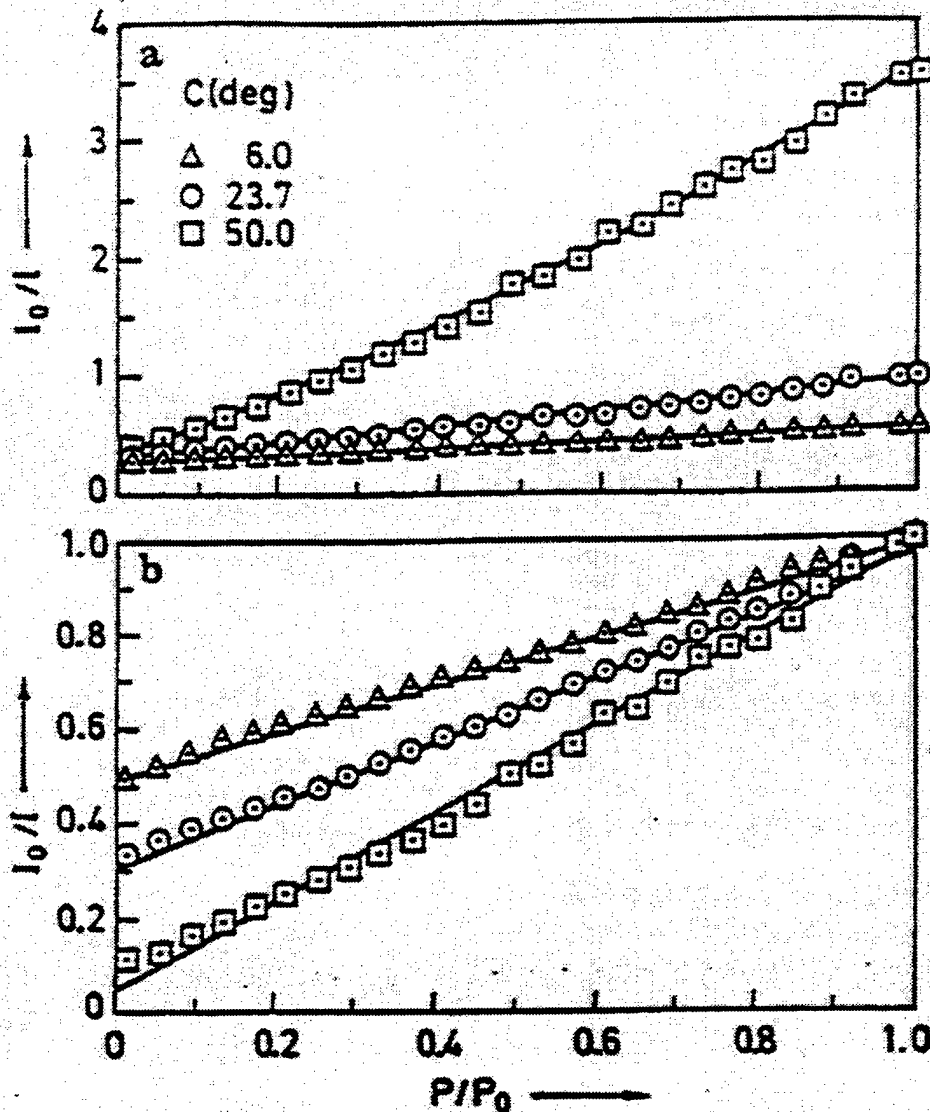
Figure 2. Effect of Temperature on Coating Calibration Curves From Kavandi [Ref. 11] (a) I_0 for Curve Measured at 23.7° C. (b) I_0 for curve taken at its Respective Temperature .
