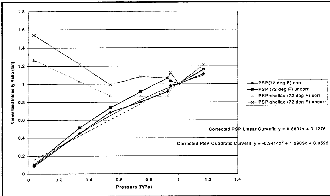
Figure F1. AC-5 Constant-Temperature, Variable-Pressure (72 0 F)
