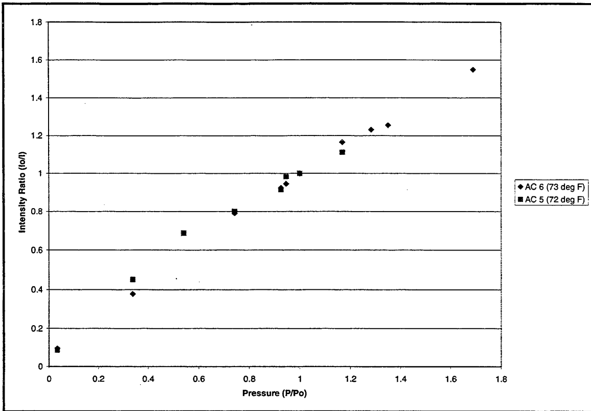
Figure 14. NPS Constant-Temperature, Variable-Pressure Repeatability (72°-73° F)
