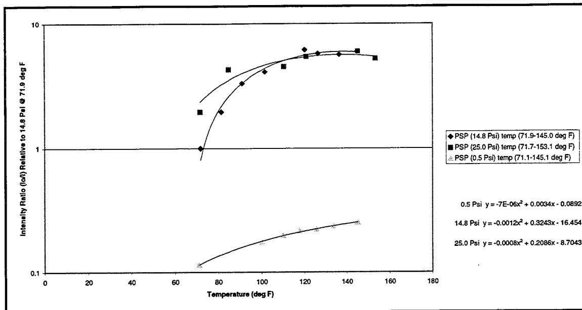
Figure 11. Constant-Pressure, Varing-Temperature Results ( I_0 at 14.8 psi and 71.9° F)
