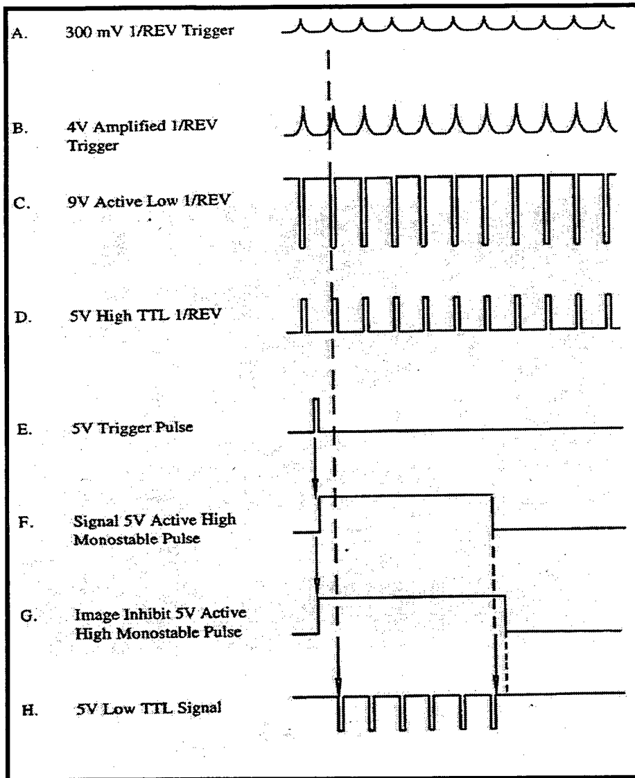
Figure 6. Image Capture Timing Sequence From Quinn [Ref. 3]
