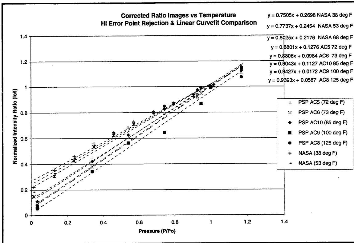
Figure 9. NPS and NASA Calibration Data with Linear Curves Fitted
