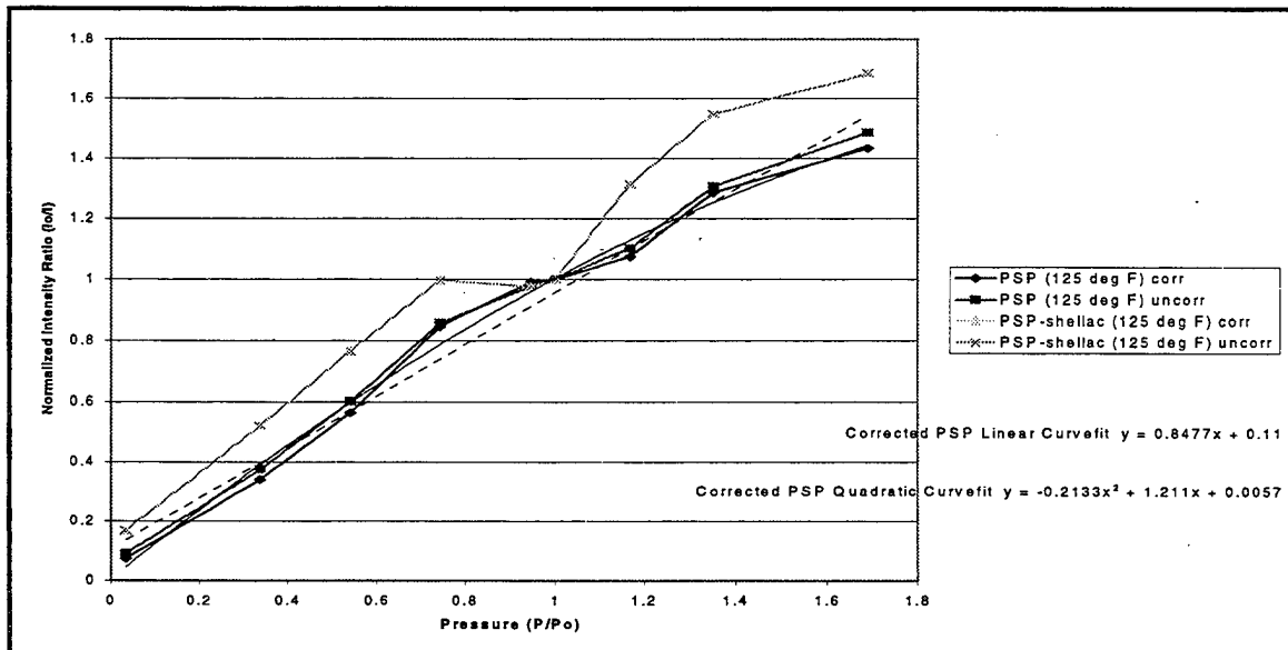
Figure F3. AC-8 Constant-Temperature, Variable-Pressure (125 0 F)
