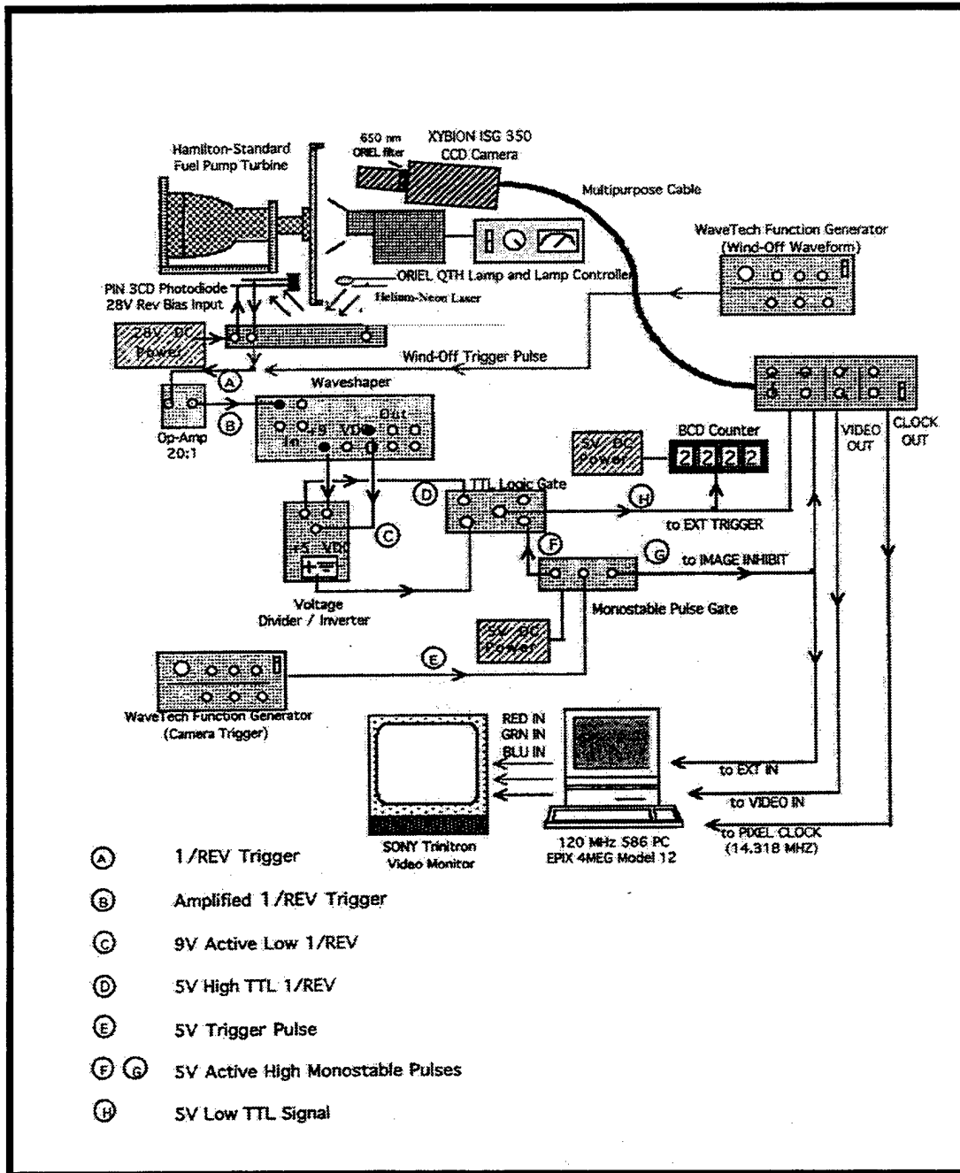
Figure 4. Image Acquisition System From Quinn [Ref. 3]
