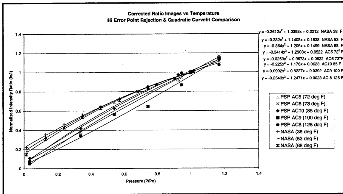
Figure 10. NPS and NASA Calibration Data with Quadratic Curves Fitted
