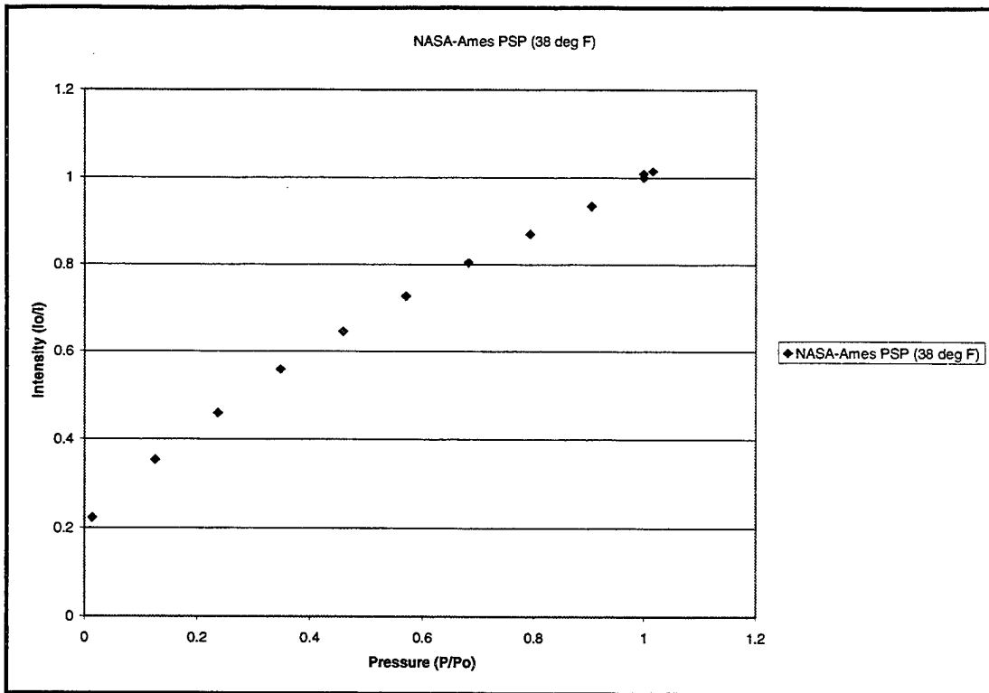
Figure D1. NASA-Ames PSP Calibration at 38° F
