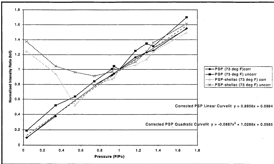
Figure F2. AC-6 Constant-Temperature, Variable-Pressure (73 0 F)
