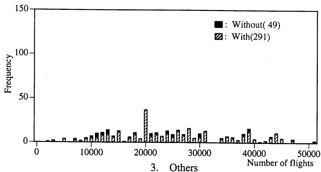
Figure 3 Relation between number of flights and frequency of detected cracks
