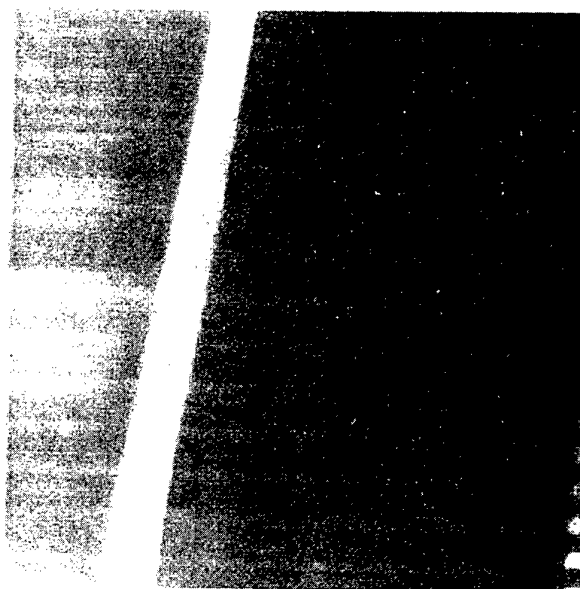
Fig. 16. Radiograph of the part of the blade with one vertical NDT-slit, 160 kV, 1.0 mA, t: 15 min, D7 film, 0.02 Pb screens, FFD: 990 mm, a: 490 mm, focus-NDT slits distance: 700 mm.
