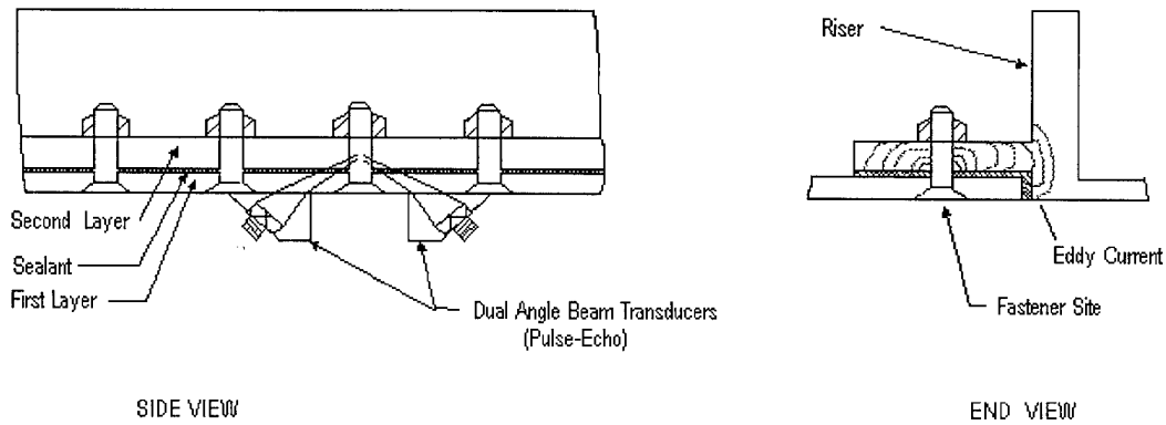
Figure 1 Splice-Joint Configuration.
