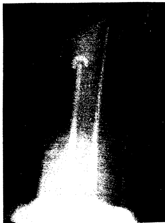
Fig. 5. Radiographic image of mottling of the gas turbine blade, with the exposure conditions: 155 kV, 1.0 mA, D7 film, 0.02 Pb screens, FFD: 360 mm, a (focus-specimen distance): 140 mm.
