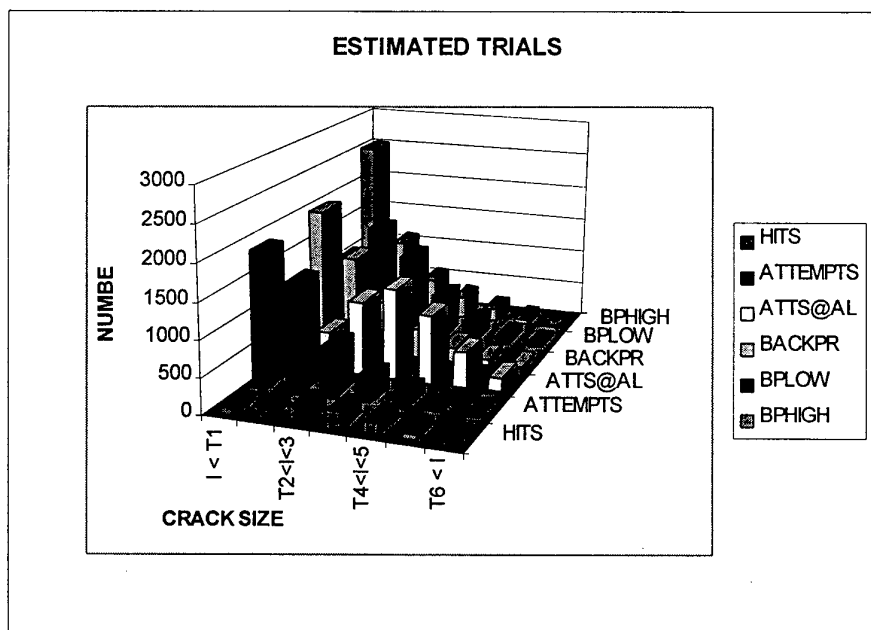
Figure 4, Estimated defect size populations for a 1000 defect simulation
