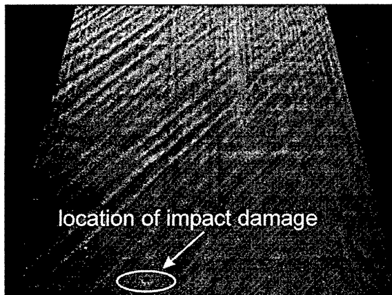
Figure 4. An example of a DAIS 500 inspection of a hat-stiffened composite panel, with a 0.006" or 0.15 mm deep impact.
