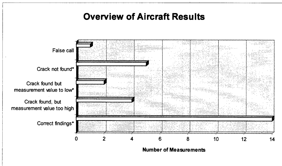
Figure 16: Results of Aircraft Inspection * Undefined flight hours between measurements can increase cracks
