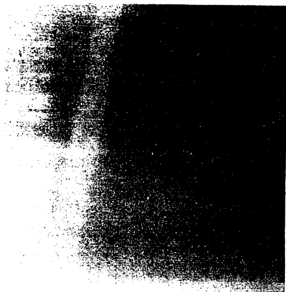
Fig. 17. Radiograph of the part of the blade with two NDT-slits in vertical and horizontal directions, 160 kV, 1.0 mA, t=15 min, D7 film, 0.02 Pb screens, FFD: 990 mm, a: 490 mm, focus-NDT-slits distance: 700 mm.
