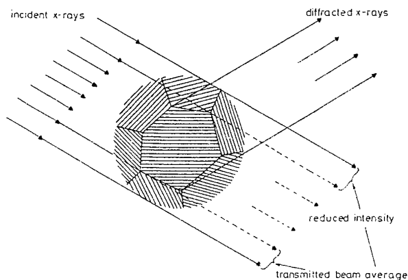
Fig. 1. Schematically explaining the reflection of some portion of the incoming X-ray from a relatively large grain.
