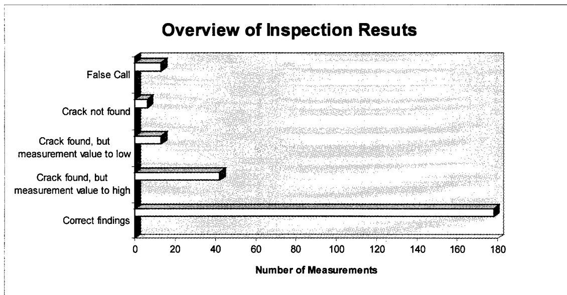
Figure 14: Results of Simulated Inspection
