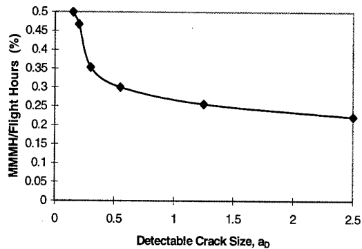
Figure 6. Influence of the detectable crack size, a_D , on cost in terms of maintenance-man-hours/flight hours for example 2.
