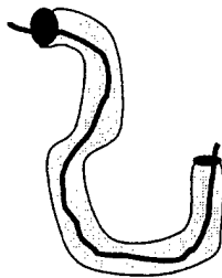
Figure 3. Reptation.
