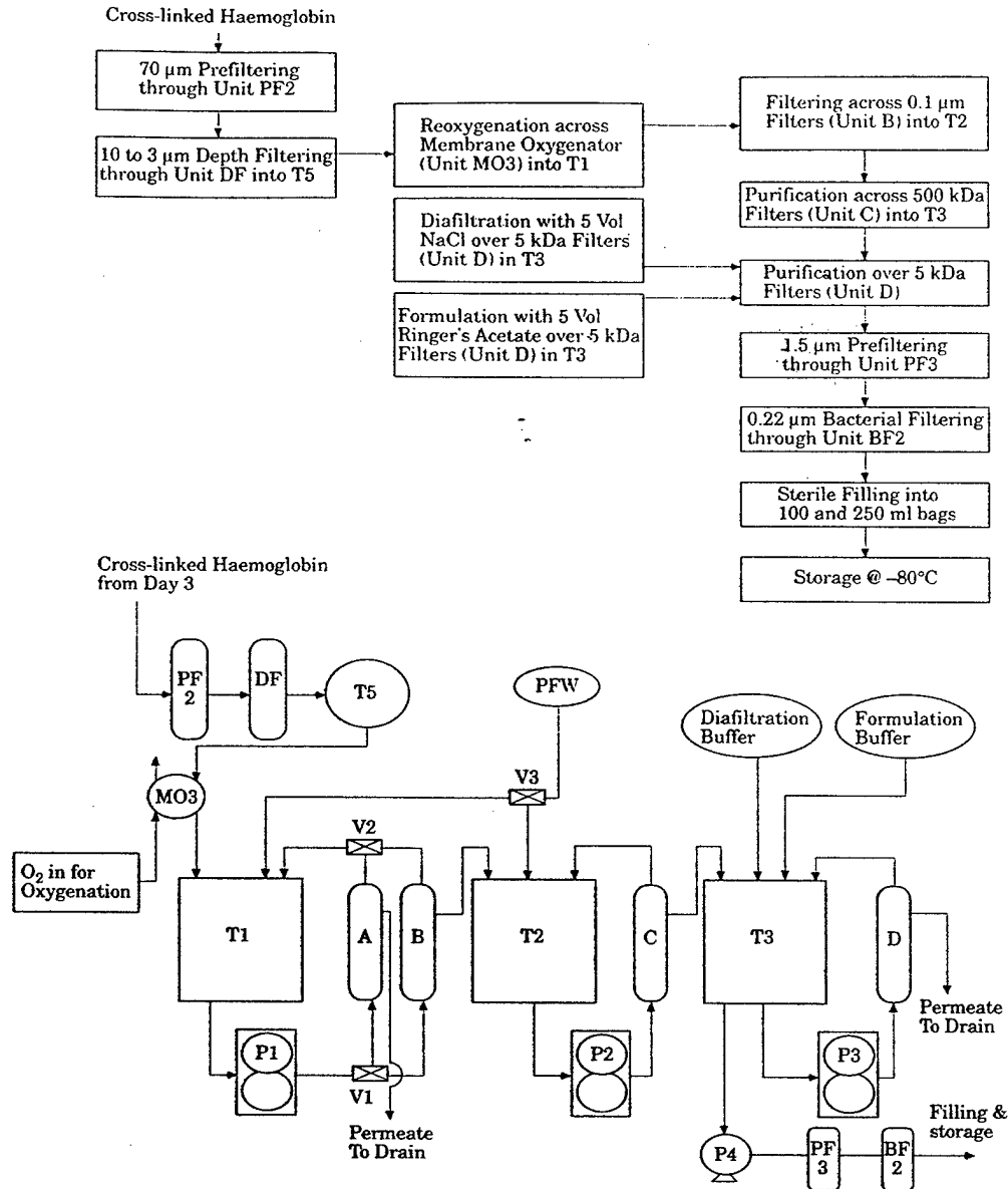
Figure 4. Process and flow diagrams for day 4. \alpha\alpha\text{Hb} is filtered stepwise through the cross flow filtration system, removing particulate matter and producing the final \alpha\alpha\text{Hb} product.
