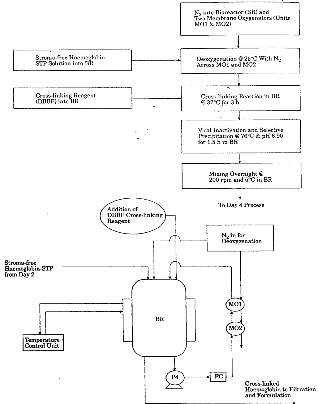
Figure 3. Process and flow diagrams for day 3. Stroma-free haemoglobin is cross-linked with DBBF, yielding \alpha\text{zHb} . Heat treatment accomplishes both pasteurization and purification of the cross-linked product.
