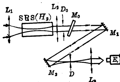
Figure 5. Experimental Arrangement Using Bicolor Mirror as the Spectroscopic Element
