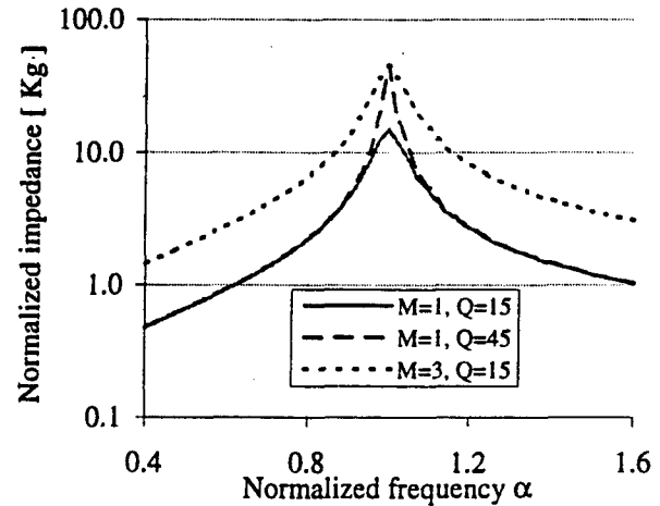
Figure 2: Normalized impedance of an ATVA
