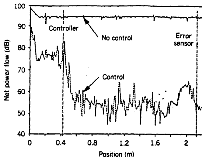
Fig. 8 Power flow distribution with and without control for the system of Fig. 7; f = 302 \text{ Hz} . 31
