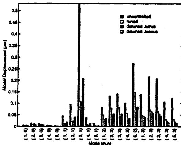
Figure 6: Structural response at 176 Hz.
