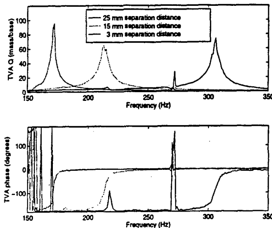
Figure 9: Different FRF of the "V" type ATVA.
