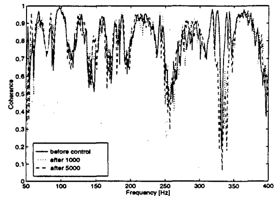
Figure 12: Coherence function \gamma_{xe}^2 before control and after 1000 and 5000 iterations using the LMS based controller.
