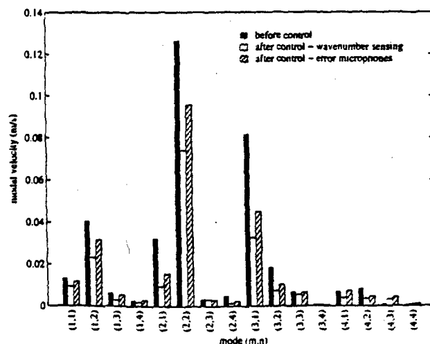
FIG. 10. Velocity modal amplitudes at 305 Hz before and after control using wave-number sensor and error microphones.
