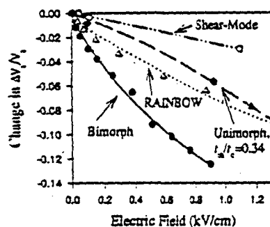
Fig. 6. Dependence of the resonant frequency \nu_r of bending vibrations on electric field. Low-field resonant frequency is: 1394 Hz (bimorph), 1015 Hz (unimorph), 595 (RAINBOW), and 236 Hz (shear-mode).
