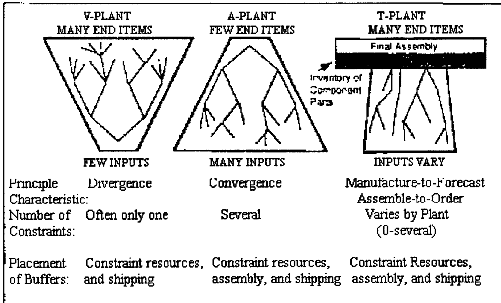
Figure 2-1: Alternative Plant Configurations
