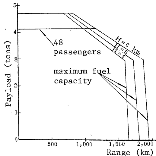
Figure 2. Payload-Range Diagram of "Y-7"
