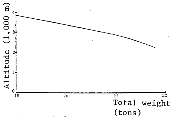
Figure 3. Single-Engine Ceiling of "Y-7"
