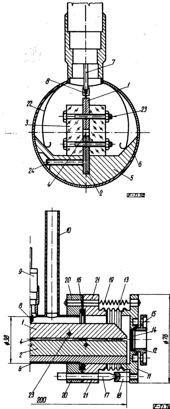
Figure 7. Longitudinal (7.a) and Cross Section (7.b) View of a Further Developed Version of the Laser
