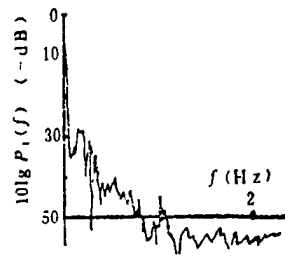
Fig. 7. Spectrum of Echo from a Slow Moving Target in Clutter After Correlation Treatment (frequency axis: 4.8828 Hz/block)
