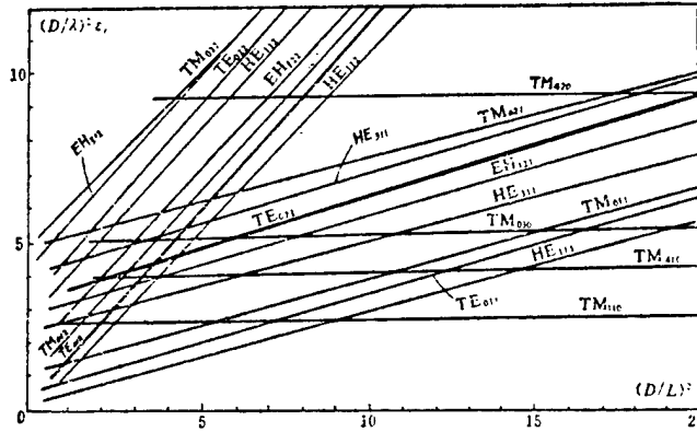
Fig. 1. Mode Patterns for Resonator with Both Ends Shorted
