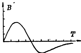
Figure 5. Waveform of measured axial magnetic field
