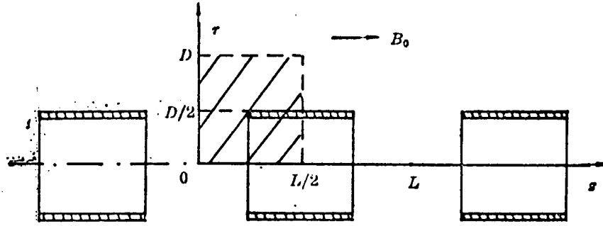
Figure 1. Cross-section view of the iron-ring wiggler. The shadowed block area is the region where computer calculation is made.
