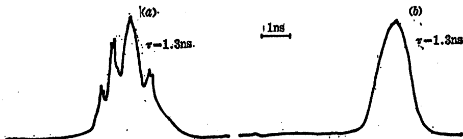
Figure 3. Temporal profiles of an ordinary Q-switched laser pulse (a) and the single-axial-mode laser pulse (b) taken by a streak camera
