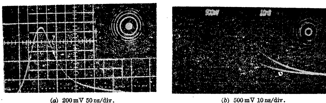
Figure 4. Spectral and temporal characteristics of the laser pulses of single axial mode (a) and double axial modes (b)
