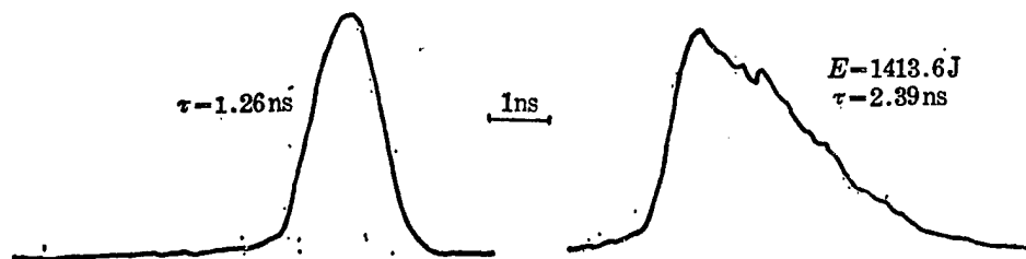
Figure 7. Sliced single-axial-mode laser pulses taken by a streak camera
