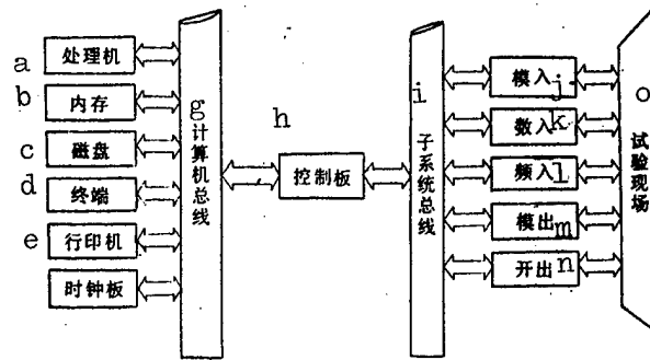
Figure 1. Hardware Environment
