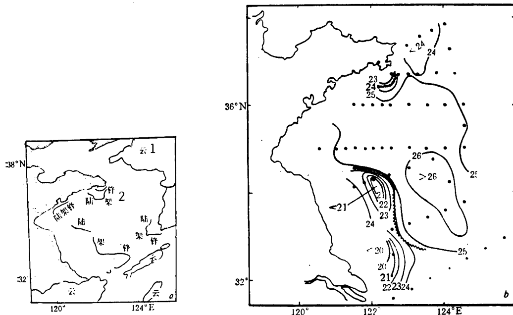
Figure 3. Distribution of the Surface Continental Shelf Front
