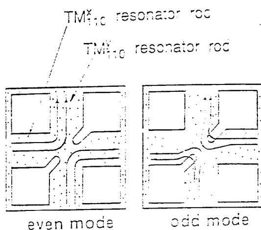
Fig.2 Electric field distribution of asymmetrically constructed orthogonal dielectric TM_{110} dual resonant mode
