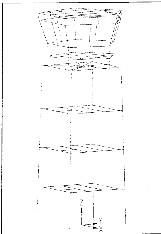
Figure 4. Finite element mesh for the 50-ft tall Salinas tower.
