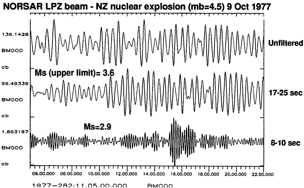
Fig. 7.3.4. NORSAR LPZ array beam recordings of a nuclear explosion ( m_b=4.5 ) at Novaya Zemlya on 9 October 1977. An unfiltered beam is shown together with the beam filtered in the "standard" 17-25 seconds band and a "high-frequency" 8-10 seconds band. Note that an interfering event masks the explosion surface waves in the 17-25 seconds band, whereas the explosion signal is clearly seen in the 8-10 seconds band.
