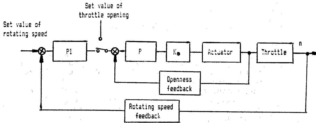
(a) Rotating speed control system
