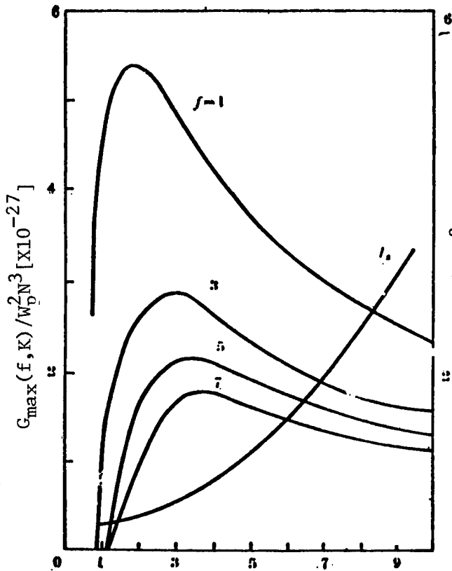
Figure 4. Gain of various harmonics versus K value when the fundamental is 5300\text{\AA} . The curve shows the injected laser power for maximum gain.
