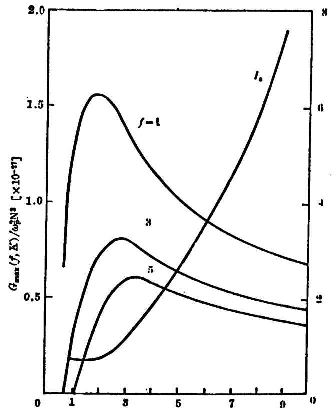
Figure 5. Gain of various harmonics versus K value when the fundamental is 1.06\mu\text{m} . The curve shows the injected laser power for maximum gain.
