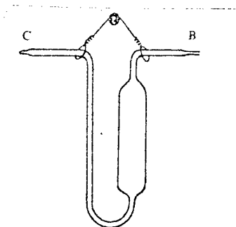
Figure 31.1: Pycnometer according to Sprengel/Ostwald.
