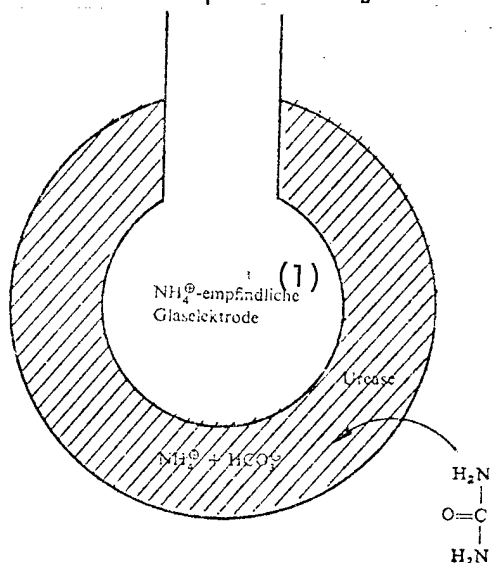
Figure 29.3. Enzyme electrode to determine urea according to the method of Guilbault [1817]. Key: (1) NH 4 sensitive glass electrode
