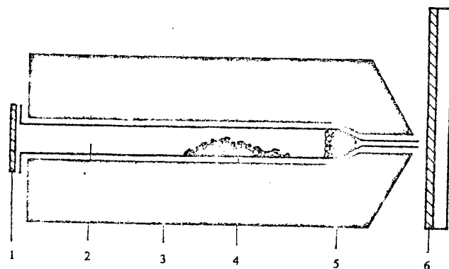
Figure 31.8: TAS Furnace Key: (1) seal; (2) glass cartridge; (3) heating block (furnace); (4) specimen; (5) glass wall; (6) DC layer.
