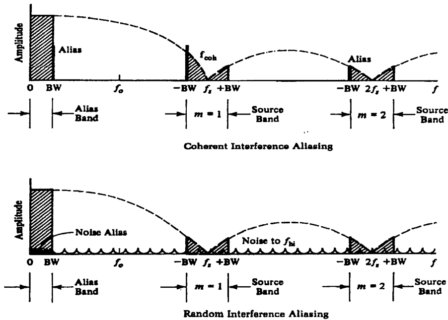
Figure 2.11 Aliasing of Coherent and Random Noise
