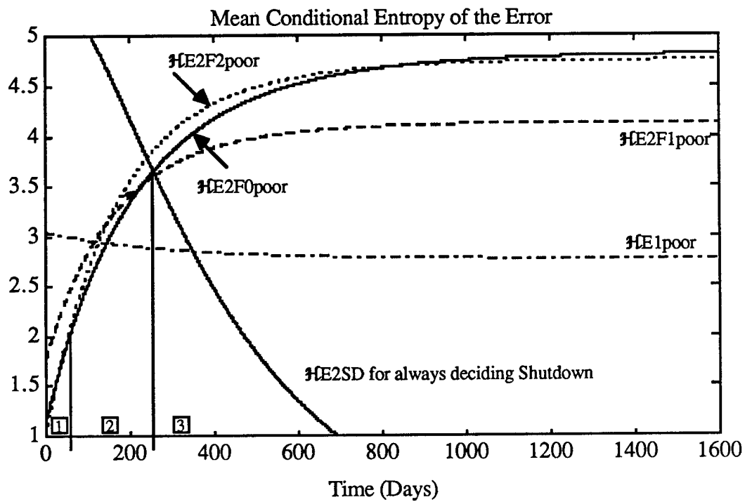
Figures 5.22 Mission Stages for Different FDI Schemes
