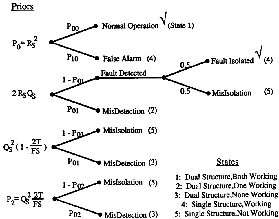
Figure 4.18 Decision Tree for FDI Scheme with Dual Redundancy
