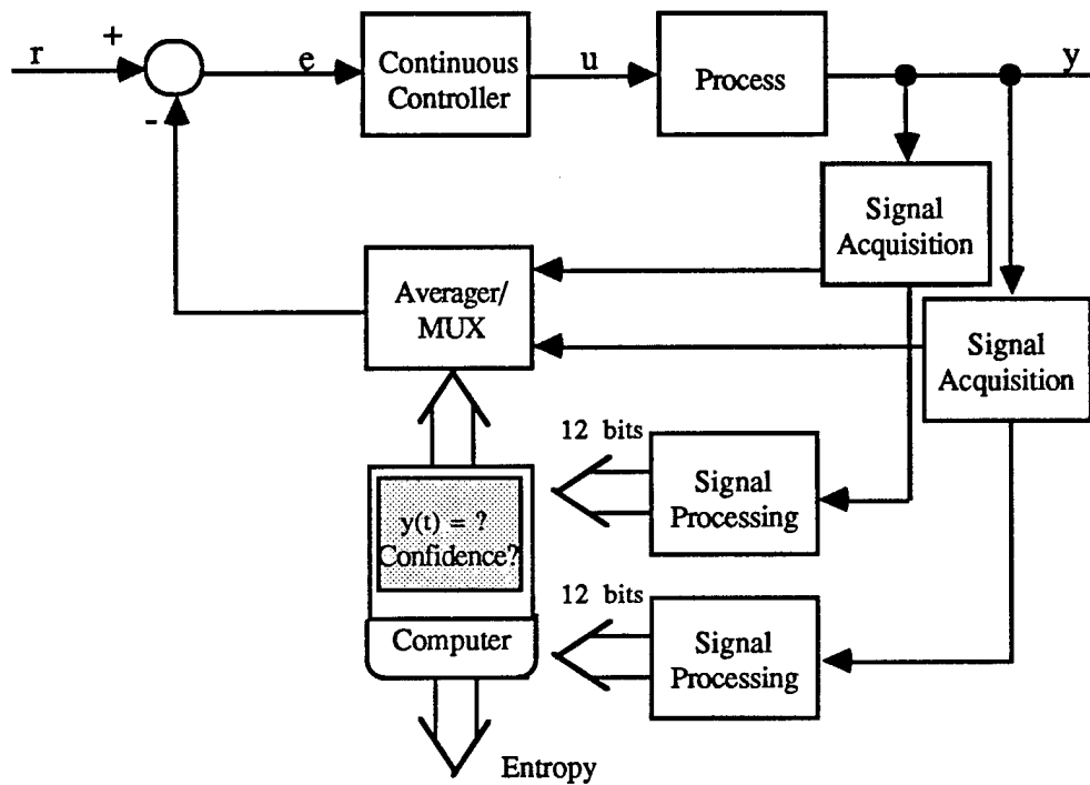
Figure 3.4 Outer Loop Observer/Planner
