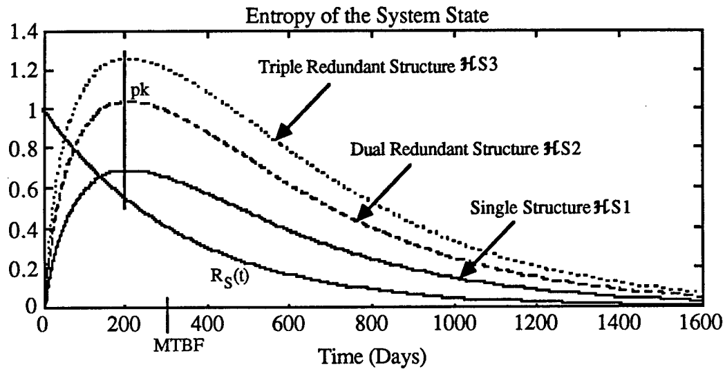
Figure 5.6 Entropy of the System State for Redundant Structures
