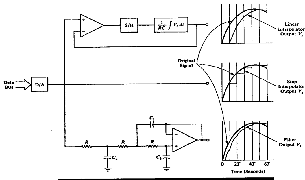
Figure 2.12 Signal Recovery Techniques
