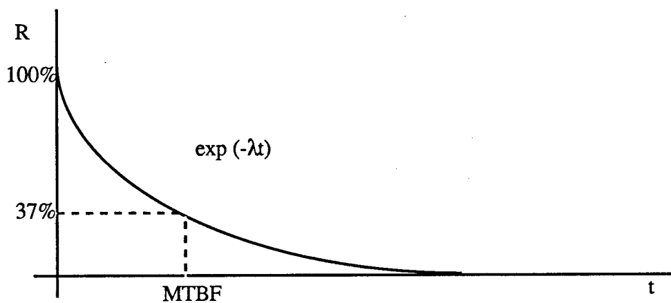
Figure 3.6 Reliability Exponential PDF during Useful Life
