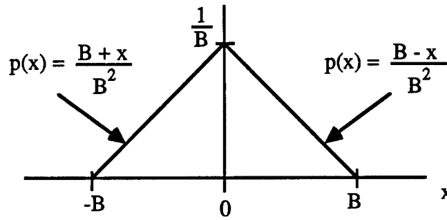
Figure 5.1 Triangular Probability Density Function
