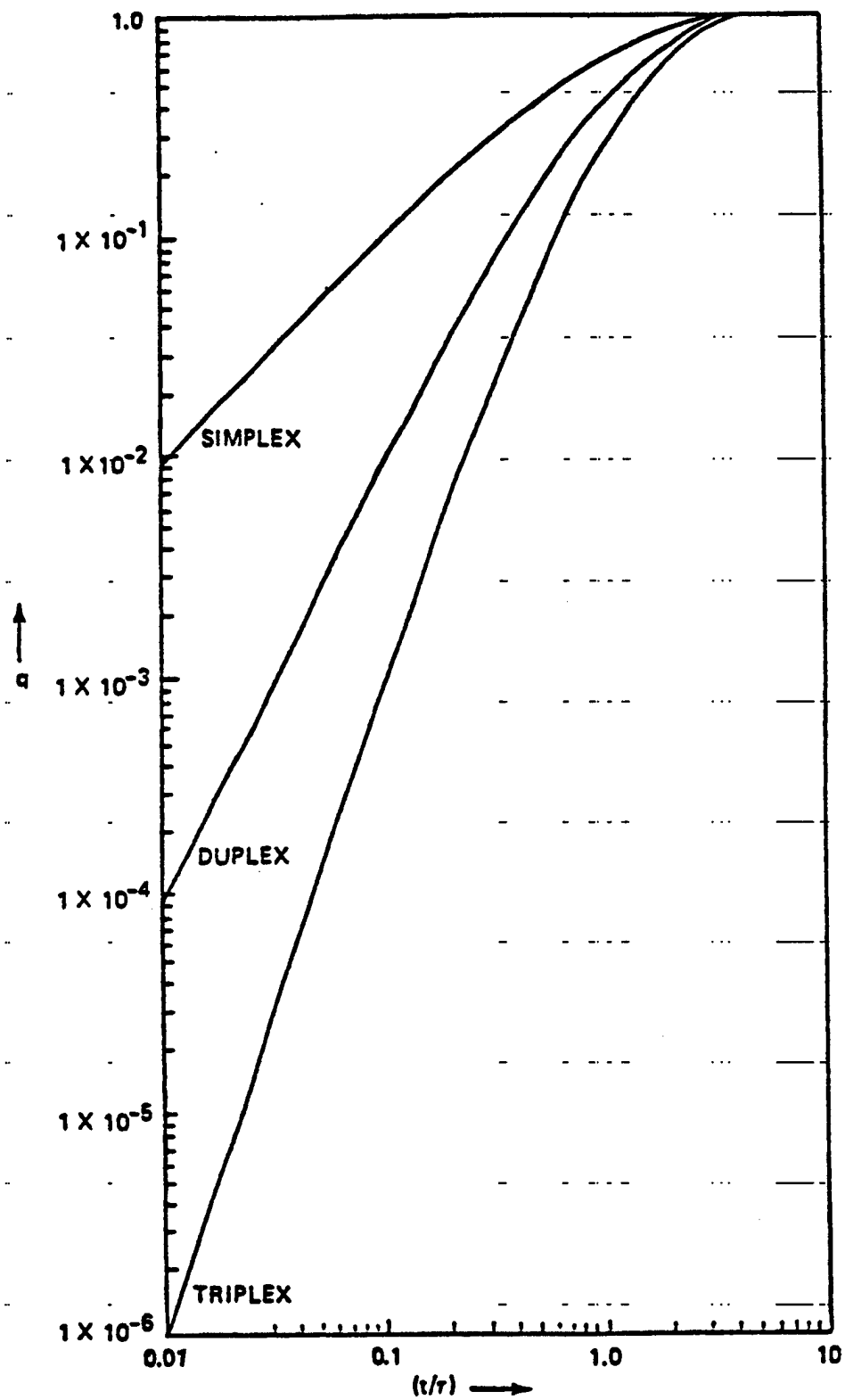
Figure 3.8 Unreliability Comparison of Redundant Configurations
