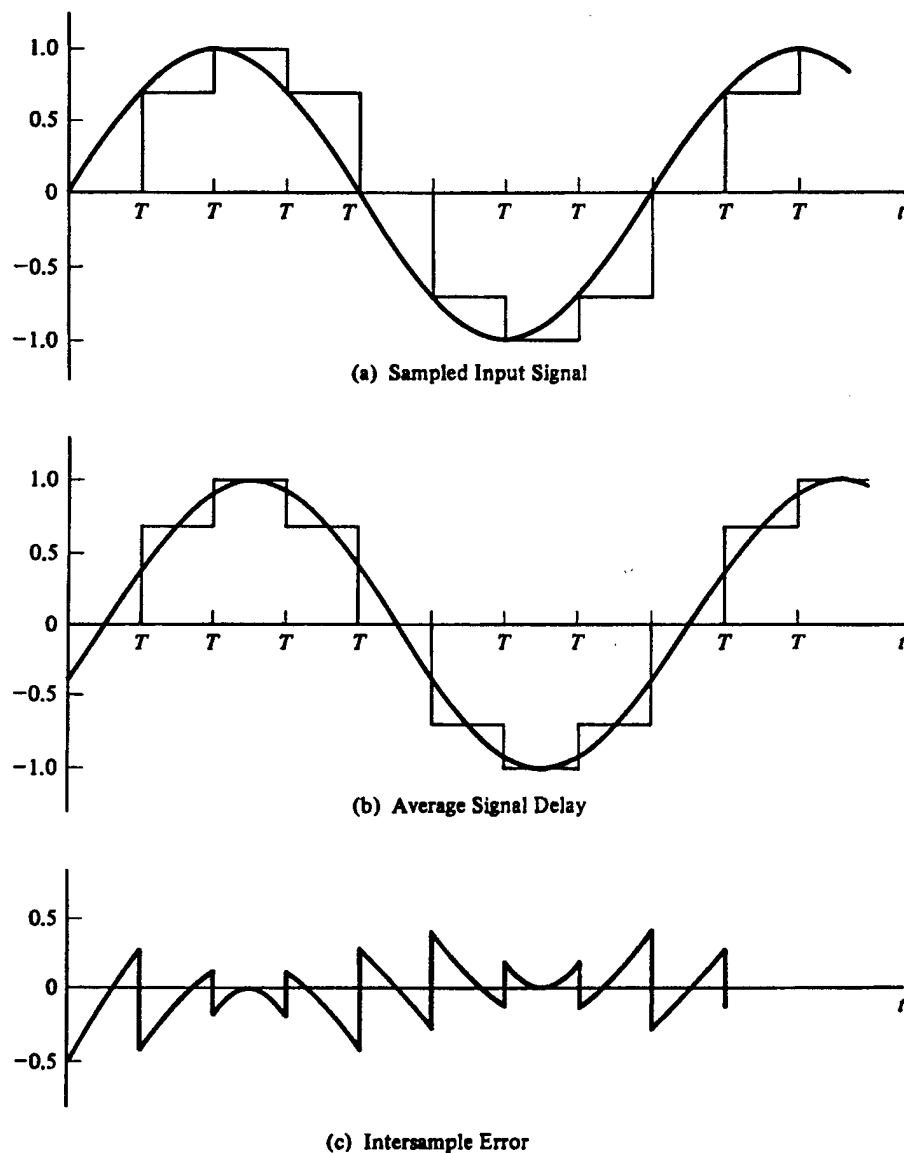
Figure 2.10 Intersample Error
