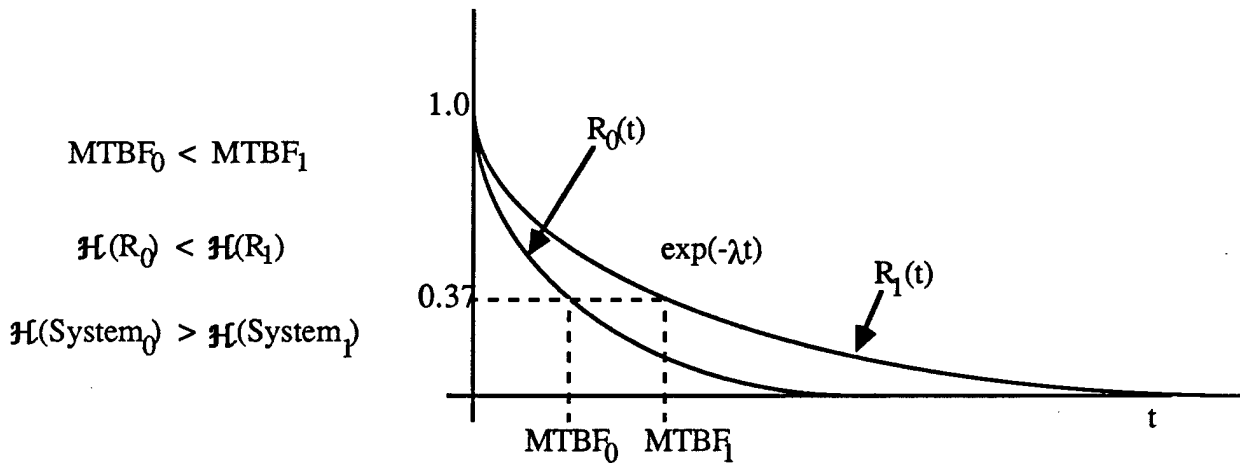
Figure 5.2 Entropy Comparison of the Reliability of Two Structures
