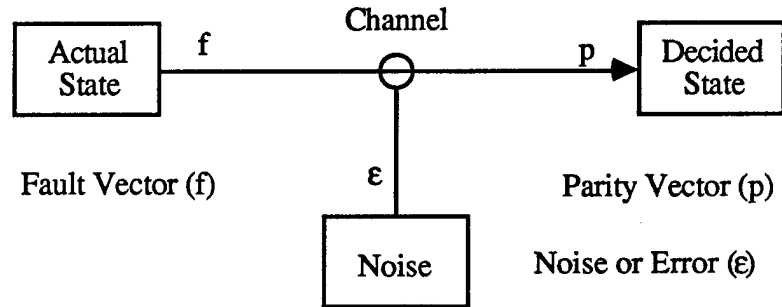
Figure 5.4 System State Decision or Information Channel
