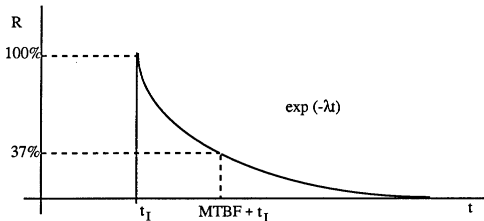
Figure 3.9 Reliability Exponential PDF after System Inspection
