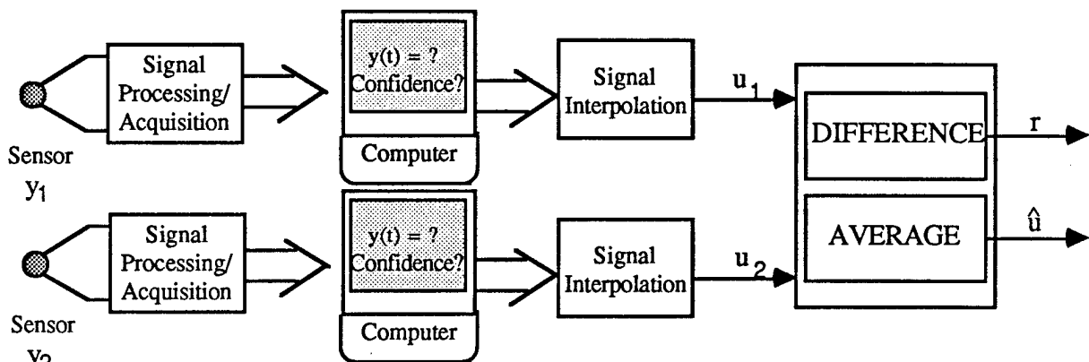
Figure 3.1 Dual-Difference Redundant Structure
