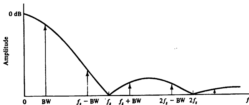
Figure 2.9 Image Spectra of Sampled Sinusoid Signal
