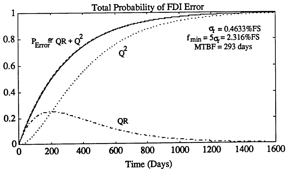
Figure 4.19 Probability of Decision Error for Optimal FDI Scheme
