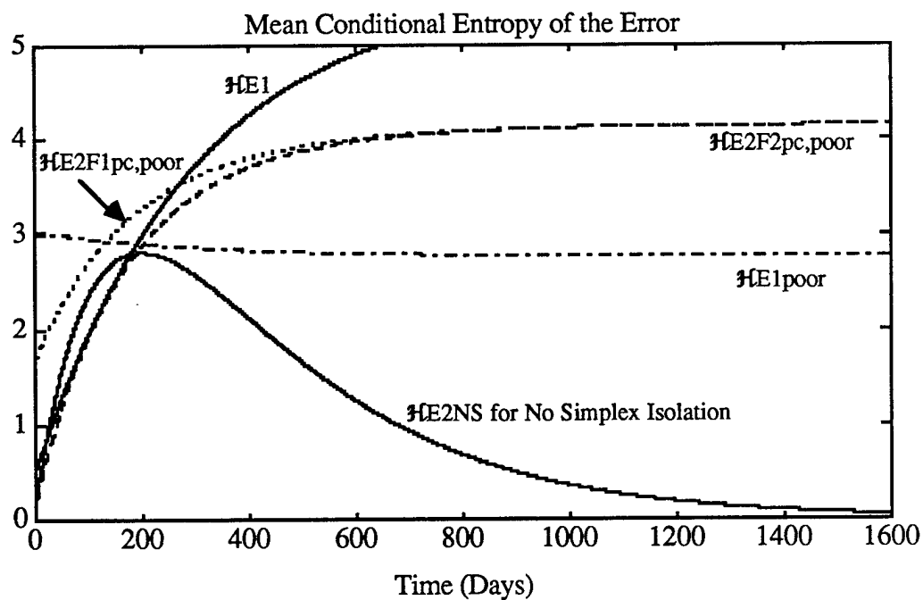
Figures 5.23 Improvement by Ignoring Poor Simplex Tests
