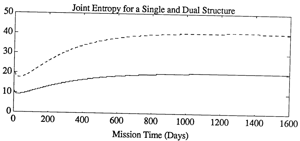
Figure B.5 Joint or System Entropy
