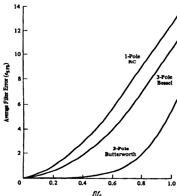
Figure 2.6 Passband Gain Deviations for Three Filters
