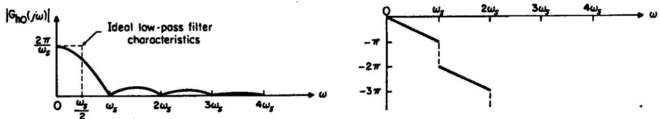
Figure 2.8 ZOH Transfer Function and Frequency Domain Representation
