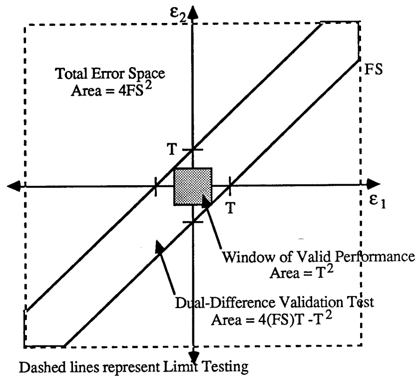
Figure 4.3 Dual-Difference Validation Space
