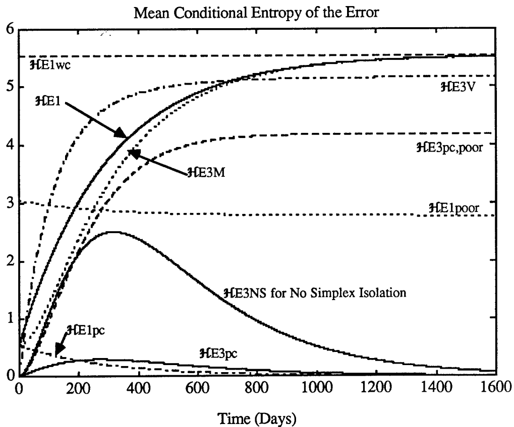
Figure 5.26 Error Entropy for Triple Structure with Shutdown and False Alarm Cost
