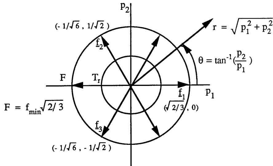
Figure 4.20 Two-Dimensional Parity Space for the TRS
