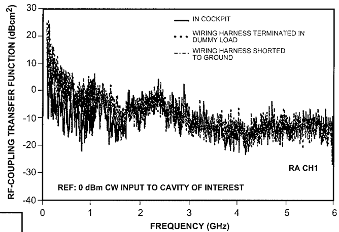
Figure 12—RF-Coupling Transfer Function for RA Channel 1 in Aircraft and on Dielectric Block in NSWCDD Reverberation Chamber
