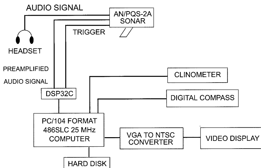
Figure 3—Block Diagram
