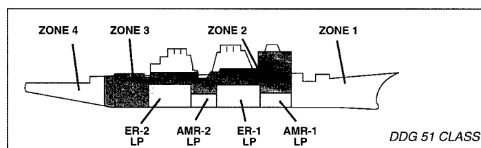
Figure 8—DDG-51 Arleigh Burke-Class Destroyer
