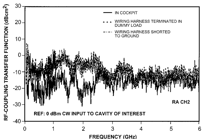
Figure 14—RF-Coupling Transfer Function for RA Channel 2 in Aircraft and on Dielectric Block in NSWCDD Reverberation Chamber
