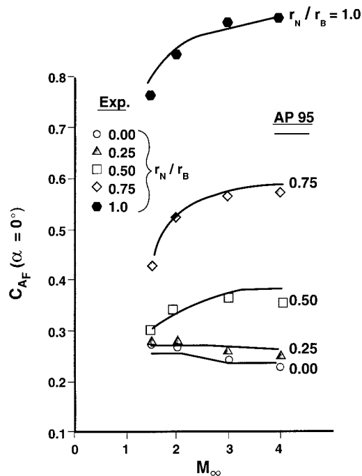
Figure 2—Variation of Forebody Axial Force Coefficient with Mach Number for Various Noses on 10-cal Afterbody ( R_N/\text{ft} = 1.8 \times 10^6 , \ell_N = 2 cal)
