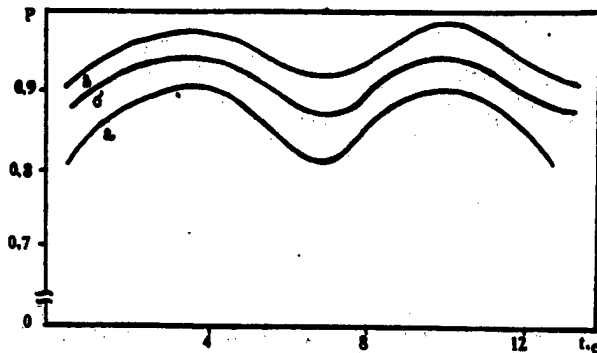
Nature of the change in the likelihood of SAM miss against airborne target depending on the time remaining until the assume moment of encounter:
