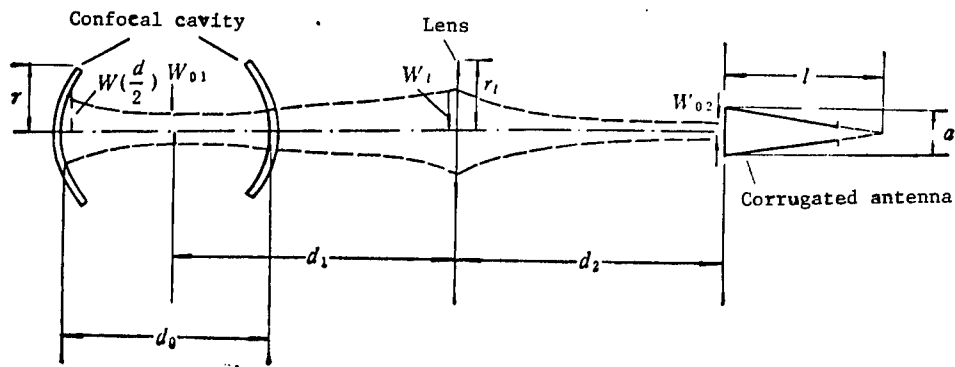
Fig. 2: Schematic of quasi-optical system
