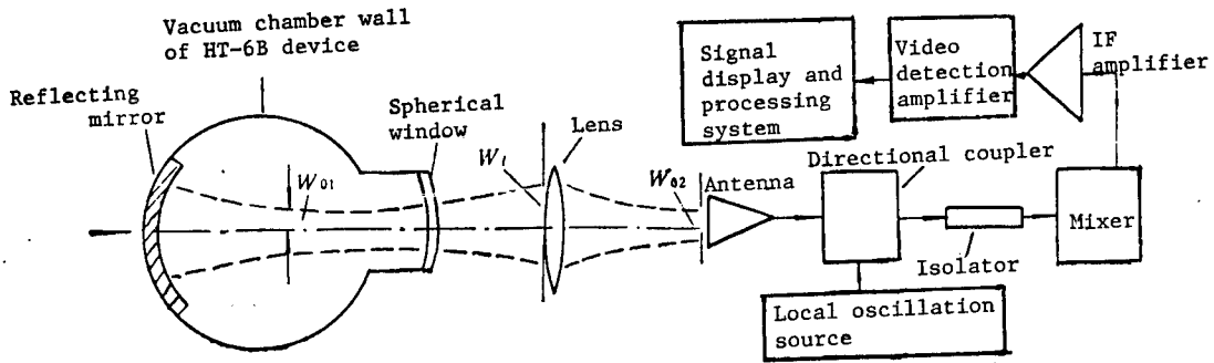
Fig. 1: Schematic of receiving system
