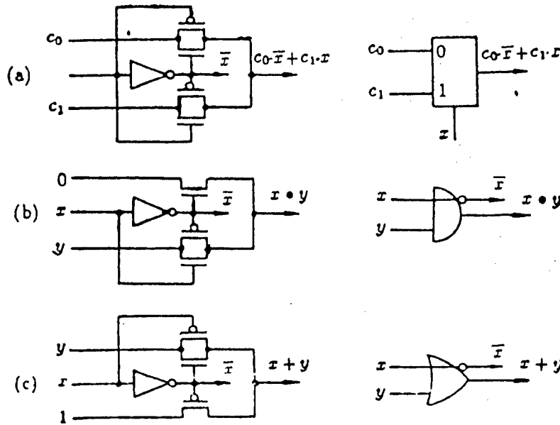
Figure 1. CMOS gates based on pass transistors: (a) 1-of-2 multiplexer, (b) AND gate, (c) OR gate.
