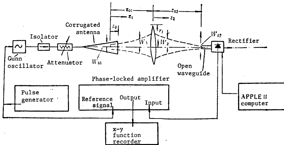
Fig. 4: Experimental arrangement of quasi-optical system for measurement
