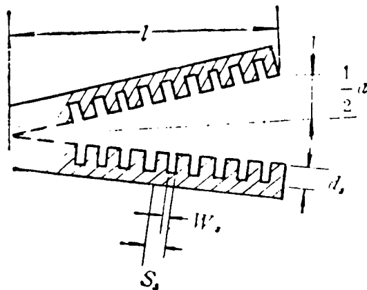
Fig. 3: Corrugated-wall circular conical horn antenna
