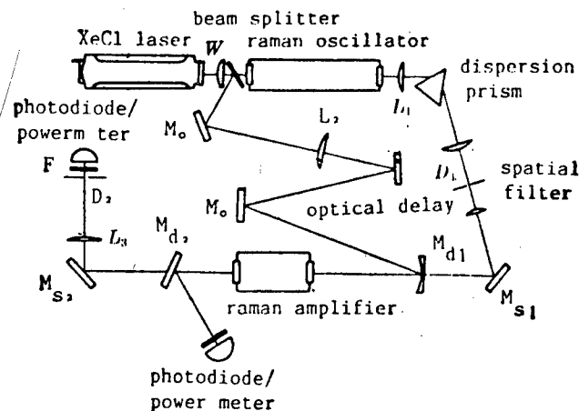
Schematic of the Raman Beam Cleanup Experiment
