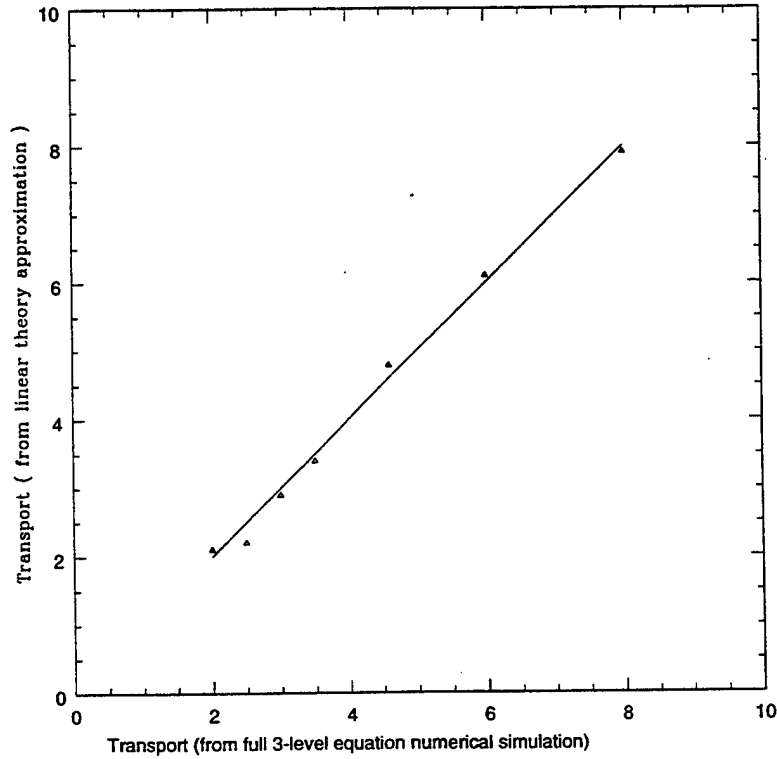
Figure 10: transports by linear theory and simulation
