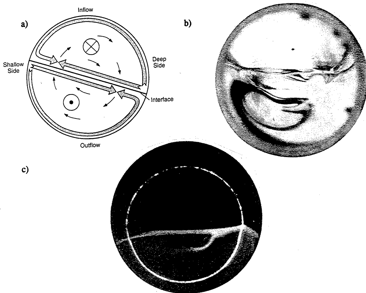
Figure 6 End views of the channel. The region - a) schematic, b) with dye streak, c) of fluorescence - shows mixing at the interface and reveals the presence of interfacial Ekman layers. The fluorescent tail extends down from the interface near the deep side and curls towards the shallow side marking the boundary between the secondary circulation. (Figure 6b viewed from the end opposite Figure 6a and 6c)
