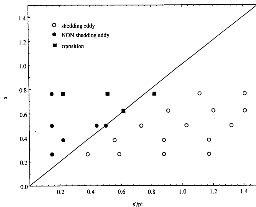
Figure 3. Regime diagram illustrating the eddy-shedding region for s \leq s'/\pi . No eddy-shedding was observed for s > s'/\pi . The squares indicate experiments where the eddy-shedding occurred after time scales much longer than in the region where s \leq s'/\pi .
