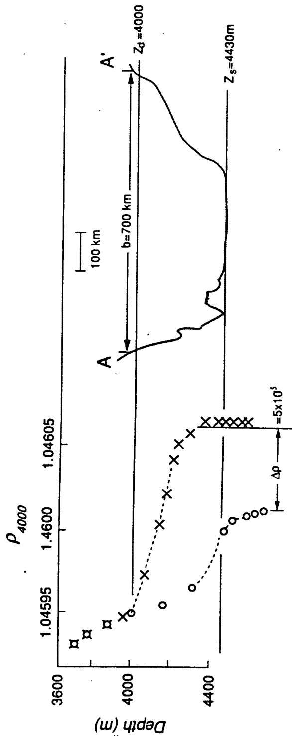
Figure 7 Estimation of \Delta \rho and H \equiv z_s - z_d for the Ceara Abyssal Plain.
