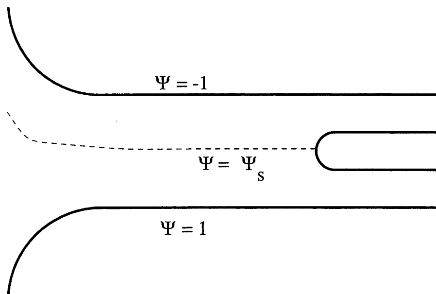
Figure 4: The geometry for rotating flow is similar to the nonrotating case in figure 1, with the addition of the streamline \Psi_s which must be determined. The total flux in the channel has also be scaled so that the streamlines on the right and left hand walls are 1 and -1 respectively.
