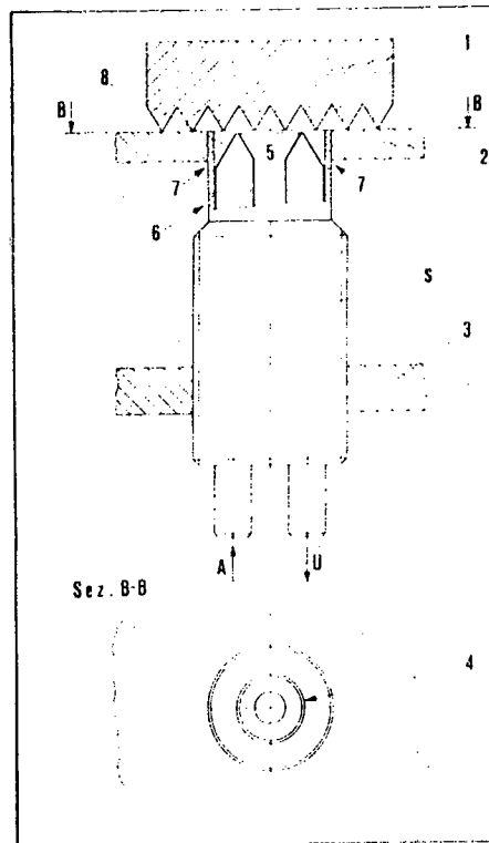
Figure 2. Sectional View of the Device With the Original Sensor
