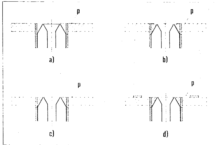
Figure 4. Different Configurations of the Sensor: a) original sensor; b) sensor with the area outside of the emitter blocked; c) sensor placed at level of support surface; d) sensor with shims for raising the object being sensed
