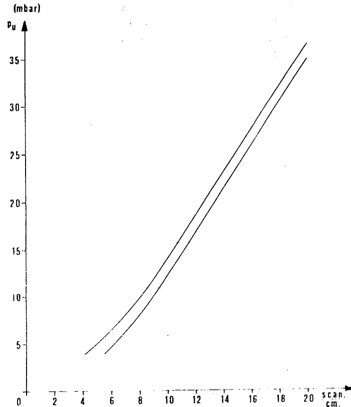
Figure 6. Maximum and Minimum Pressure Values for Sensor Placed at Level of Test Support Surface
