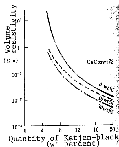
Figure 5. Electric Conductivity of Polypropylene Added With Ketjen Black EC and Calcium Carbonate
