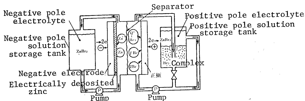
Figure 3. Principle Drawing of Zinc Bromide Battery (Charging status)
