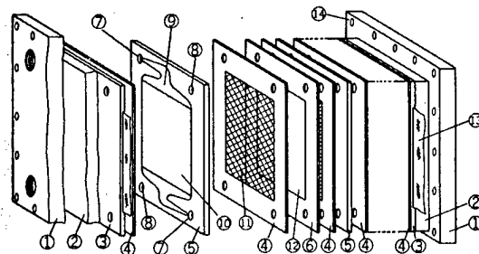
Figure 4. Elements and Construction of Layer-Built Battery
