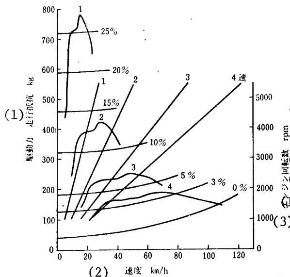
Chart 7. Predicted Driving Performance Curve
