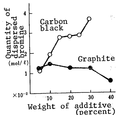
Figure 7. Quantity of Bromine Dispersion After 250 Hours
