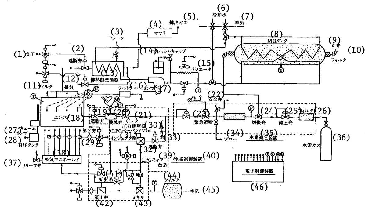
Chart 4. Control system
