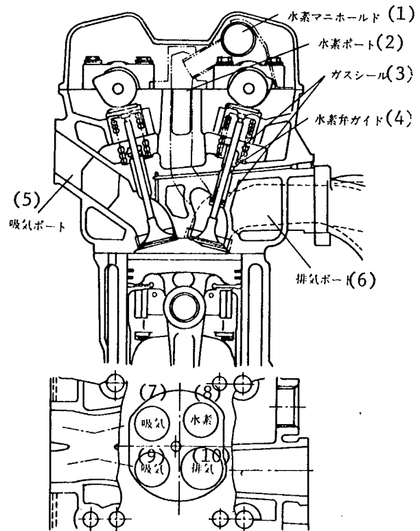
Chart 2. Outline of the experimental cylinder head
