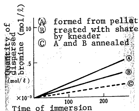
Figure 6. Bromine Dispersion in High Density Polyethylene
