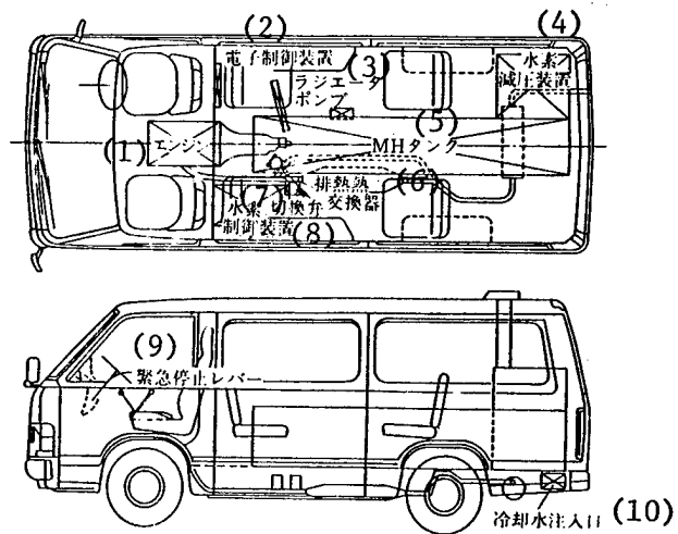
Chart 6. Configuration of components in the car
