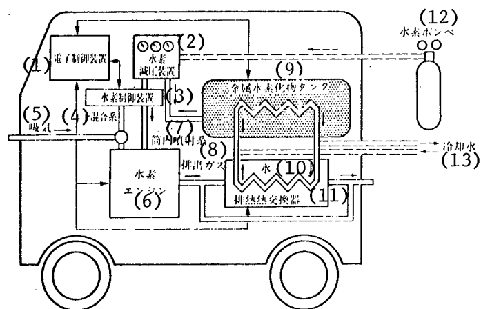
Chart 1. Structure of Hydrogen-fueled Car
