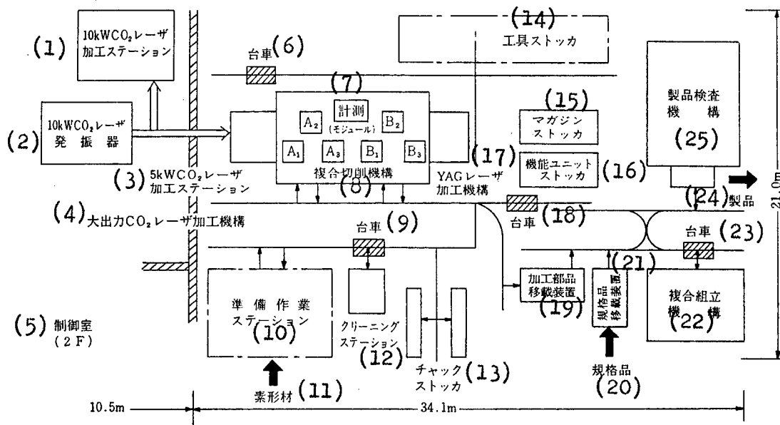
Figure 2. System Organization and Product Flow in the Experimental Plant
