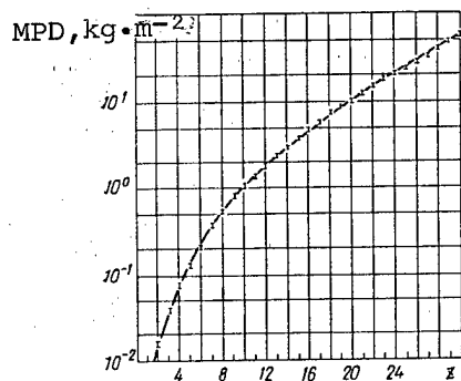
Figure 1. MPD as a function of particle charge Z
