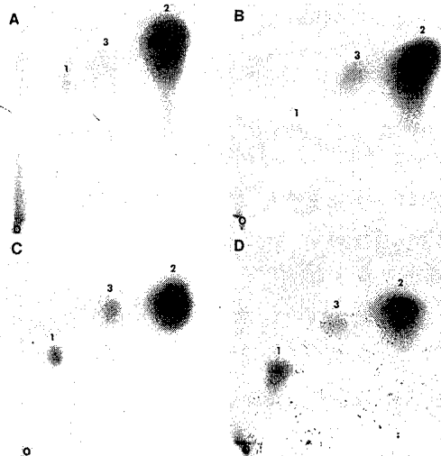
FIG. 1. Autoradiograms showing PhIP-DNA adduct patterns obtained by incubating 20 \mu mol/L N-OH-PhIP with 2 mg/mL of calf thymus DNA in the presence of (A) 1 mmol/L acetyl CoA; (B) 1 mmol/L adenosine triphosphate (ATP); (C) 0.2 mmol/L PAPS; and (D) 100 \mu mol/L arachidonic acid. Incubations A, B, and C were with 1 mg/mL cytosolic protein from human breast tissue, and incubation D was with 1 mg/mL of microsomal protein from breast tissue. O is the chromatographic origin. Adducts are assigned number 1, 2, and 3 based on previous studies. 10,11,14,15 Adducts were not observed in negative control reactions without cofactors for matching autoradiography exposure times.
