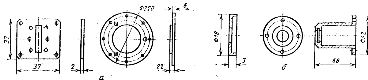
Figure 1. Examples of geometrically different parts with the same names and part numbers per NO.000.05 MNSChKh: a - flange (XX8.230.XXX per MNSChKh); б - bushing (XX8.223.XXX per MNSChKh)
