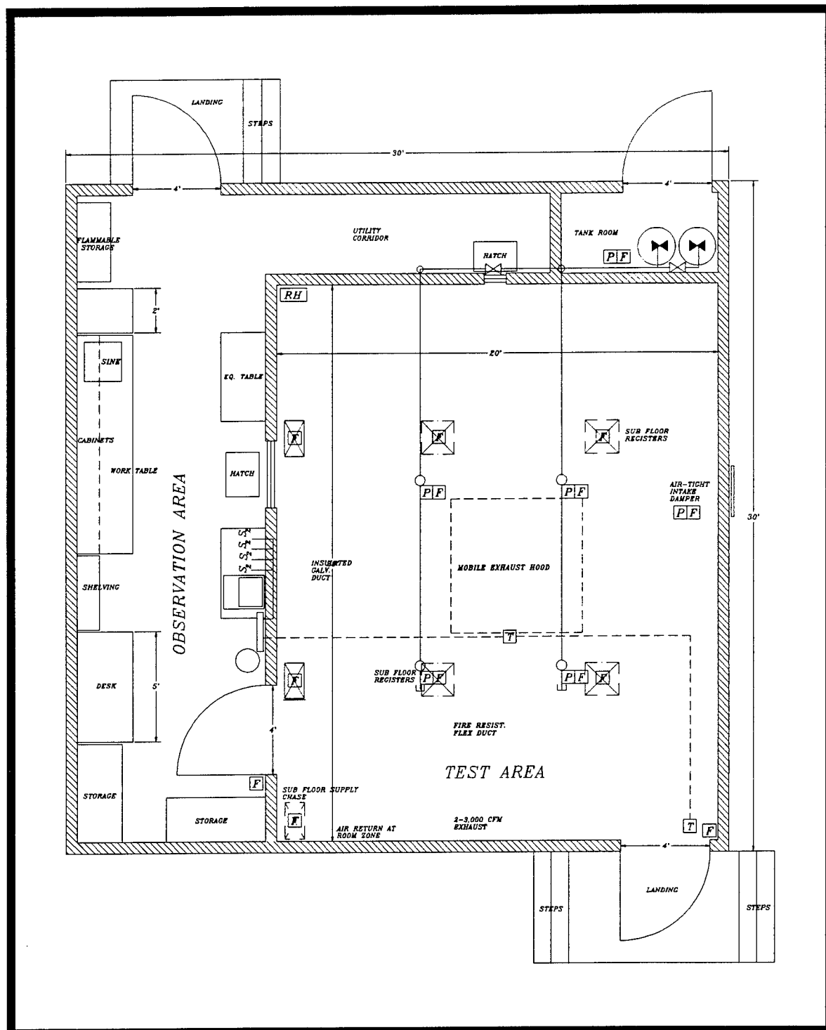
Figure 3 Test cell instrumentation and support equipment layout.
