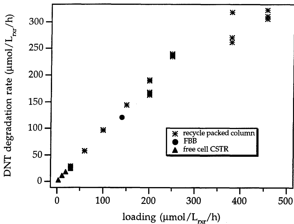
Figure 12. Comparison of performance of FBB run of Fig. 11 to other reactors(10).
