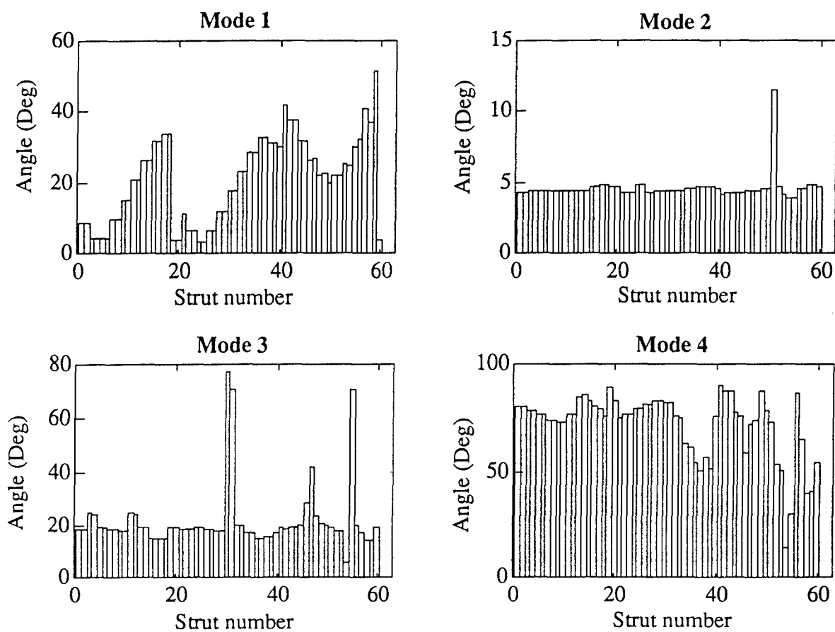
Fig. 7 Damage location results of damage case D
