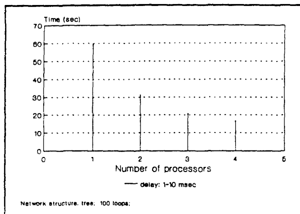
Figure 5. Test Program Execution Times
