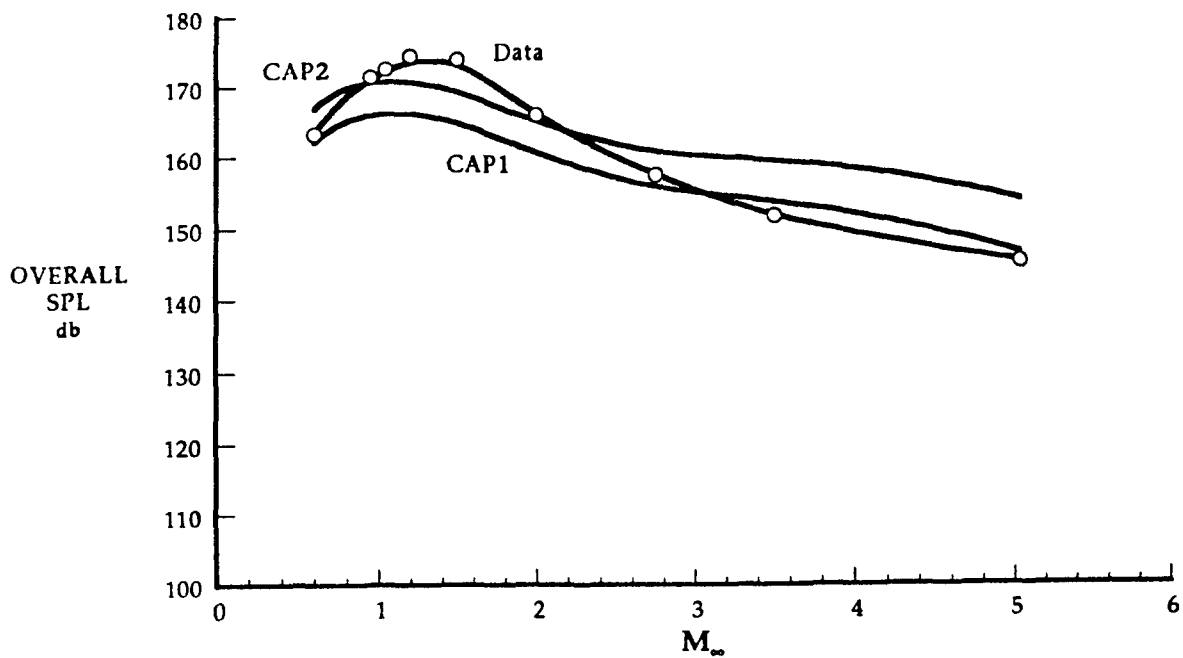
a. Overall Sound Pressure Level (OASPL)
