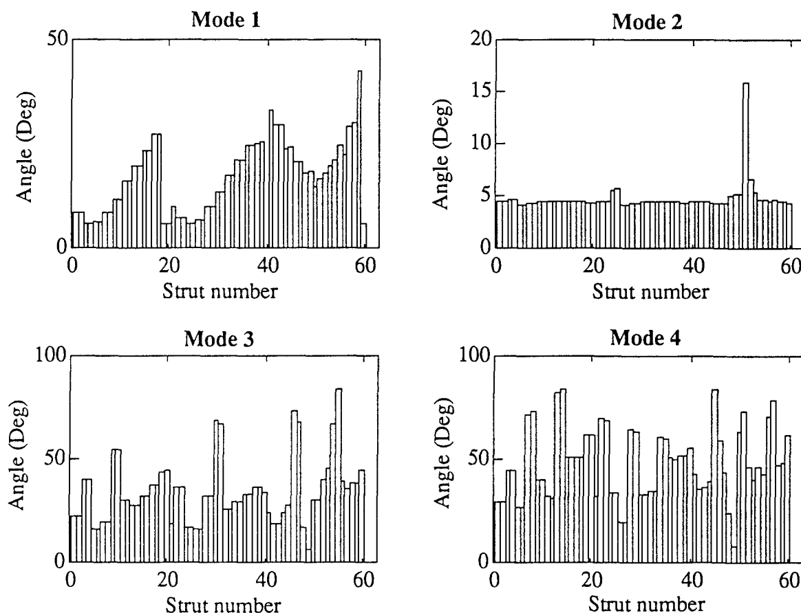
Fig. 6 Damage location results of damage case C
