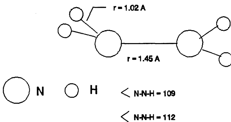
FIGURE 1: Geometry of Hydrazine
