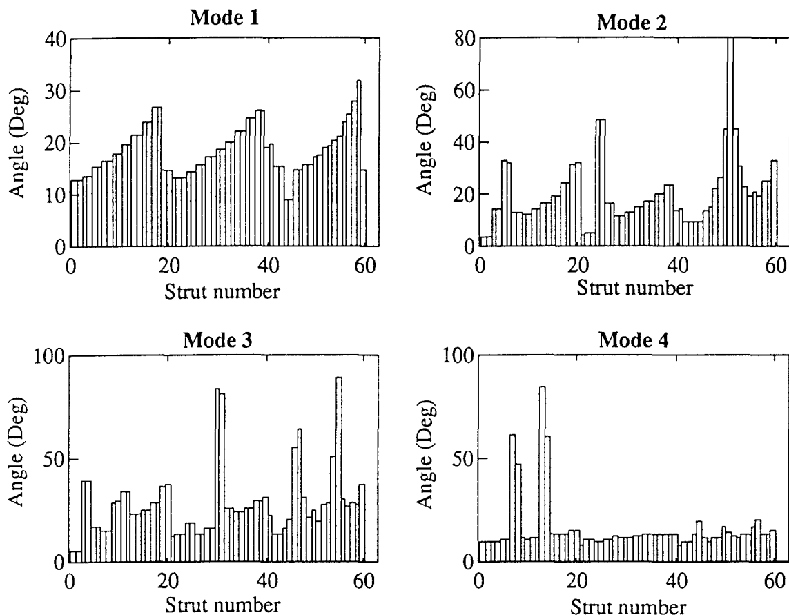
Fig. 4 Damage location results of damage case A
