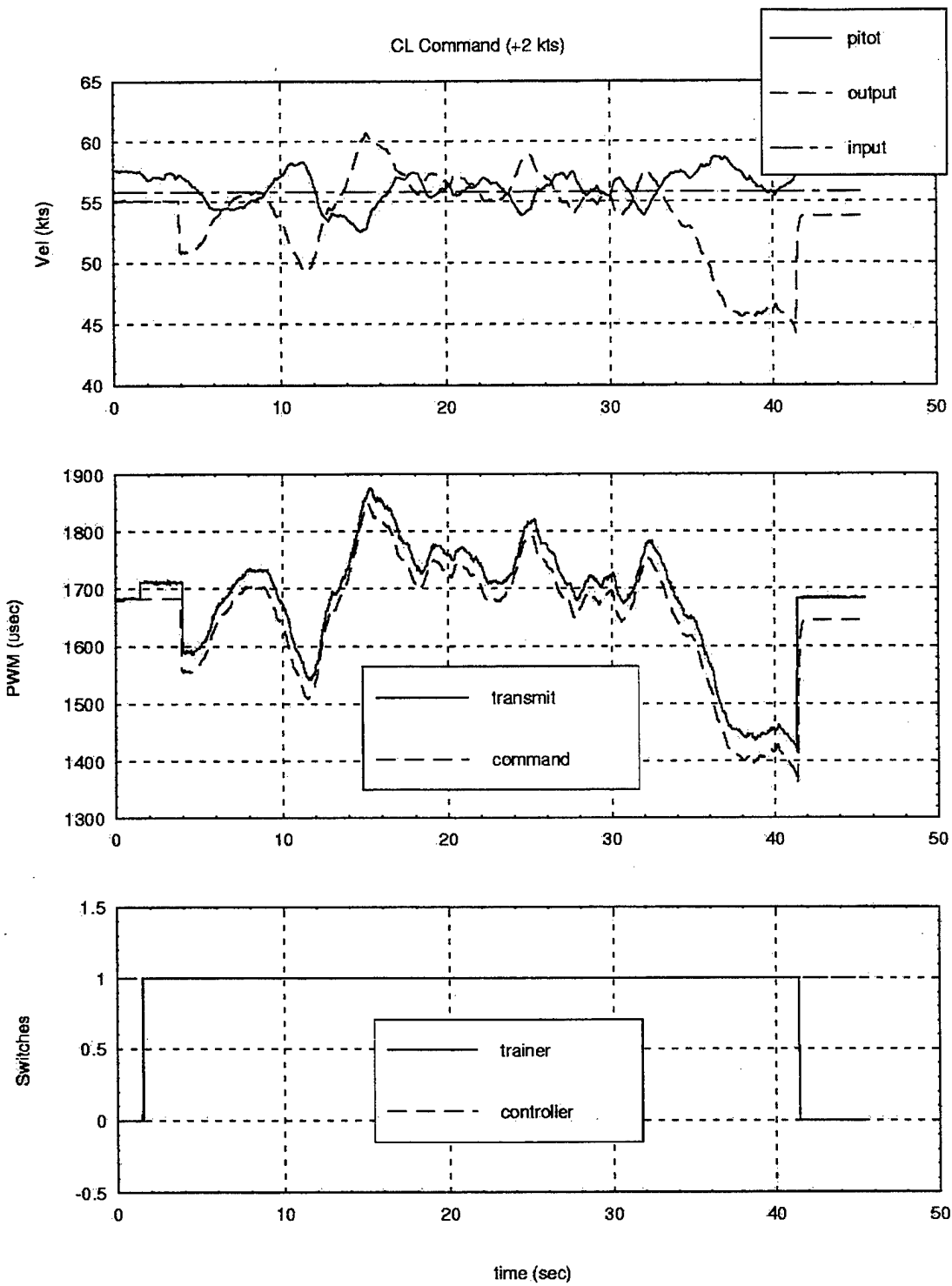
Figure 5.3: CL Airspeed Command
