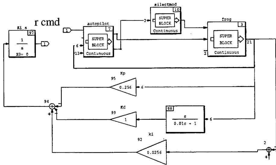
Figure 4.9: Control Loop
