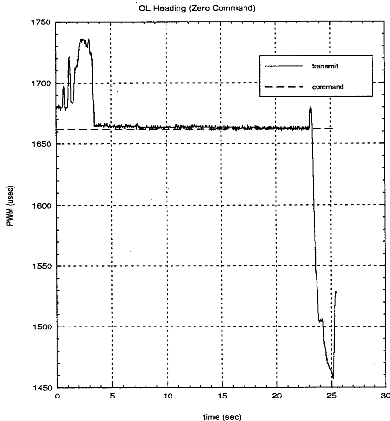
Figure 5.9: OL Heading Command Calibration
