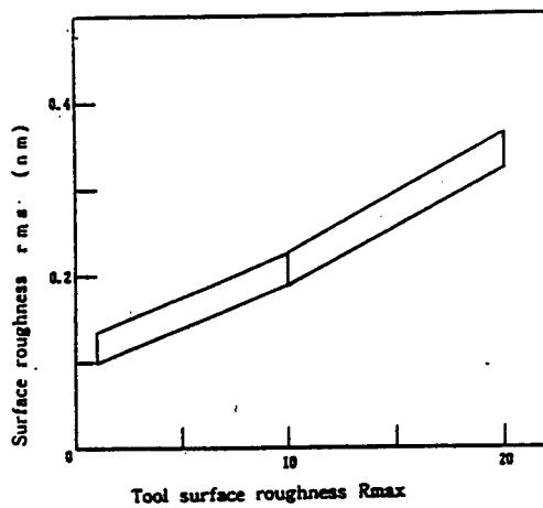
Fig.A6 Correlation with tool surface roughness
