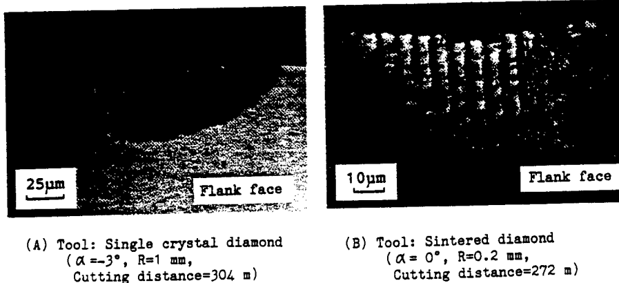
Fig.9 Photographs of worn flank faces of cutting tools. (Cutting speed = 170\text{ m/min} , Feed rate = 5\text{ }\mu\text{m/rev} , Depth of cut = 1\text{ }\mu\text{m} )
