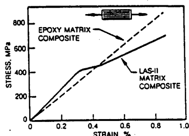
Figure 6 Tensile Stress Strain Curve for Unidirectional SiC Composites.
