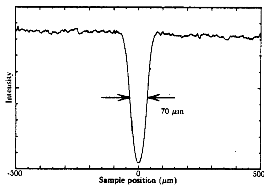
Fig. 3. Diffracted signal intensity versus sample position x in the LIG measurement. The probe delay time was fixed at \tau_d = 100 \text{ psec} . At 2 h before the measurement, the spot at x = 0 had been annealed for a few hours.
