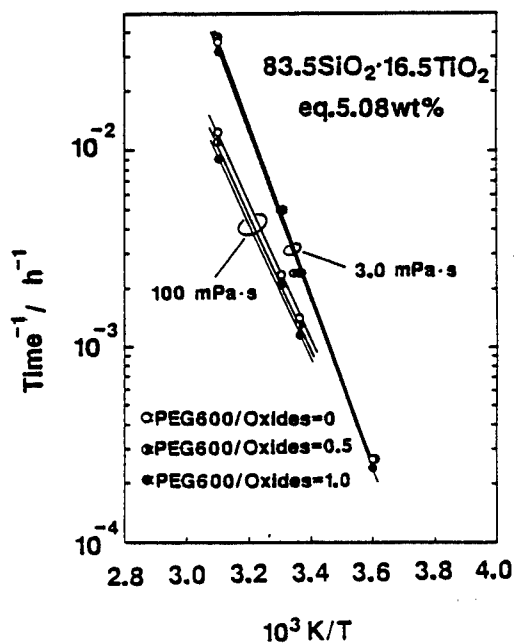
Fig. 7. Temperature dependencies of the inverse of the time at which the viscosity of the sols becomes a given value, 3.0 and 100 mPa·s. Open, half-closed and closed circles have the same meanings as in Fig. 6.
