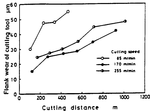
Fig.11 Effect of cutting distance on flank wear of cutting tool. (Tool: Sintered diamond, \alpha = 0^\circ , R = 0.2 mm, Feed rate = 5 μm/rev, Depth of cut = 1 μm)
