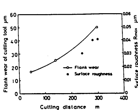
Fig.10 Effects of cutting distance on flank wear of cutting tool and surface roughness. (Tool: Single crystal diamond, \alpha = -3^\circ , R = 1 mm, Cutting speed = 170 m/min, Feed rate = 5 μm/rev, Depth of cut = 1 μm)
