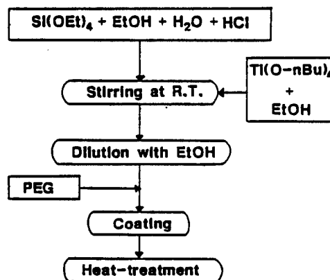
Fig.2. Preparation procedure of polyethylene glycol(PEG)-containing SiO 2 -TiO 2 solutions.
