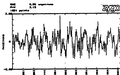
Fig. A9 Polished Surface Roughness Measured by ZYGO HP5500
