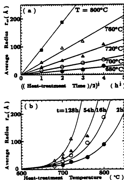
FIG. 1. (a) heat treatment time dependence. Heat treatment time t is set at 2, 16, 54, or 128 h. Temperature T is set at 680, 700, 720, 760, or 800 °C. The solid lines are fitted to the experimental data using the minimum squares method. The measurement error of the average radius is 20%. (b) heat treatment temperature dependence. The solid lines are the calculated curves for each heat treatment time using the equation r_{av} = r_0(t) \exp[\beta(t)T] .
