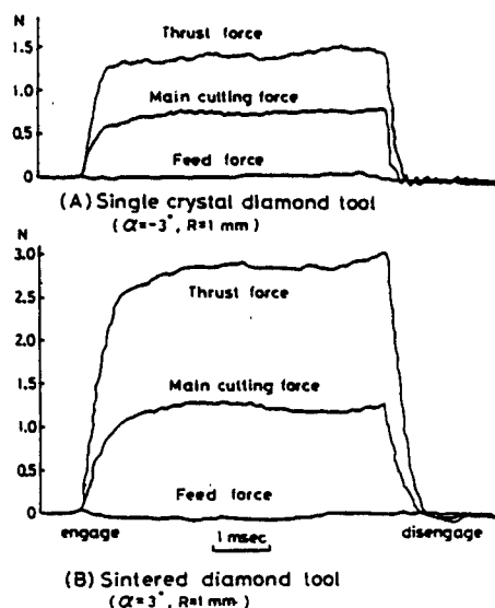
Fig.3 Example of cutting force components measure. (Cutting speed=170 m/min, Feed rate=5 \mu m/rev, Depth of cut=1 \mu m)
