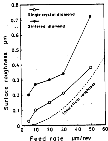
Fig.5 Effect of feed rate on surface roughness. (Tool: Single crystal diamond, \alpha=3^\circ , R=1 \text{ mm} and Sintered diamond, \alpha=-3^\circ , R=1 \text{ mm} , Cutting speed= 170 \text{ m/min} , Depth of cut= 1 \mu\text{m} )
