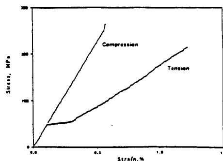
Figure 8 Stress-Strain Curves of Tension and Compression for chopped Graphite Fiber Reinforced Glass Composites
