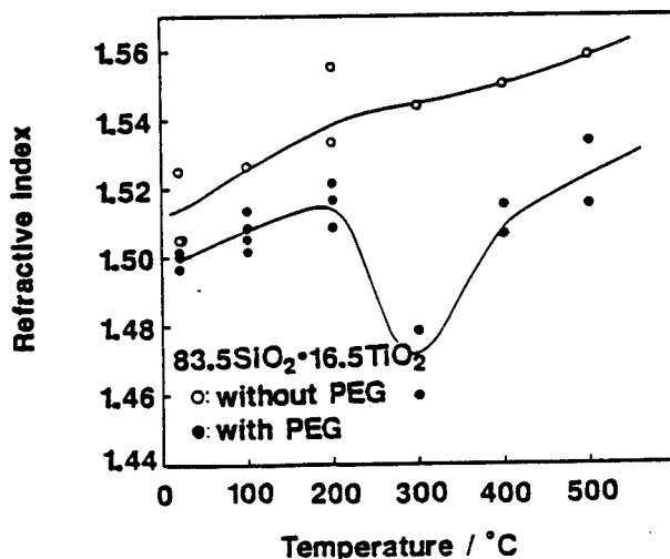
Fig.4. Variations of refractive index of 83.5\text{SiO}_2 \cdot 16.5\text{TiO}_2 films with heat-treatment; open and closed circles are respectively for the films obtained without PEG and with the addition of PEG. The weight ratio of PEG600 added to oxides is unity.
