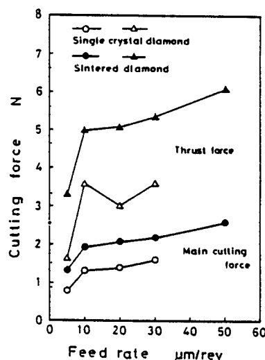
Fig.4 Effect of feed rate on cutting forces. (Tool: Single crystal diamond, \alpha = 3^\circ , R = 1 mm and Sintered diamond, \alpha = -3^\circ , R = 1 mm, Cutting speed=170 m/min, Depth of cut=1 \mu m)
