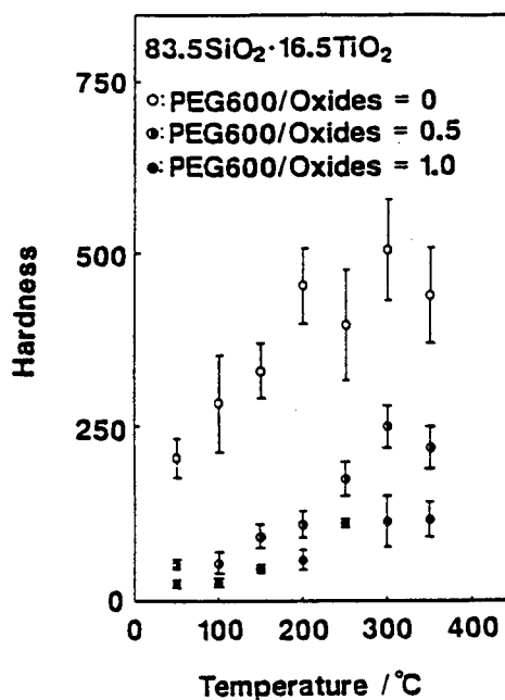
Fig. 8. Comparison of hardness of the films containing different amounts of PEG600 as a function of heat-treatment temperature. Open, half-closed and closed circles represent PEG600/oxides weight ratio = 0, 0.5 and 1.0, respectively.
