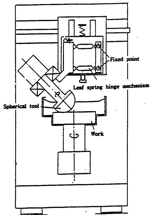
Fig.2 Polishing Device.
