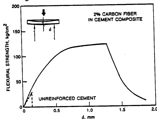
Figure 1 Comparison of Bend Tests for Unreinforced Cement and Cement Matrix Composites Containing 2% of Chopped Carbon Fiber.
