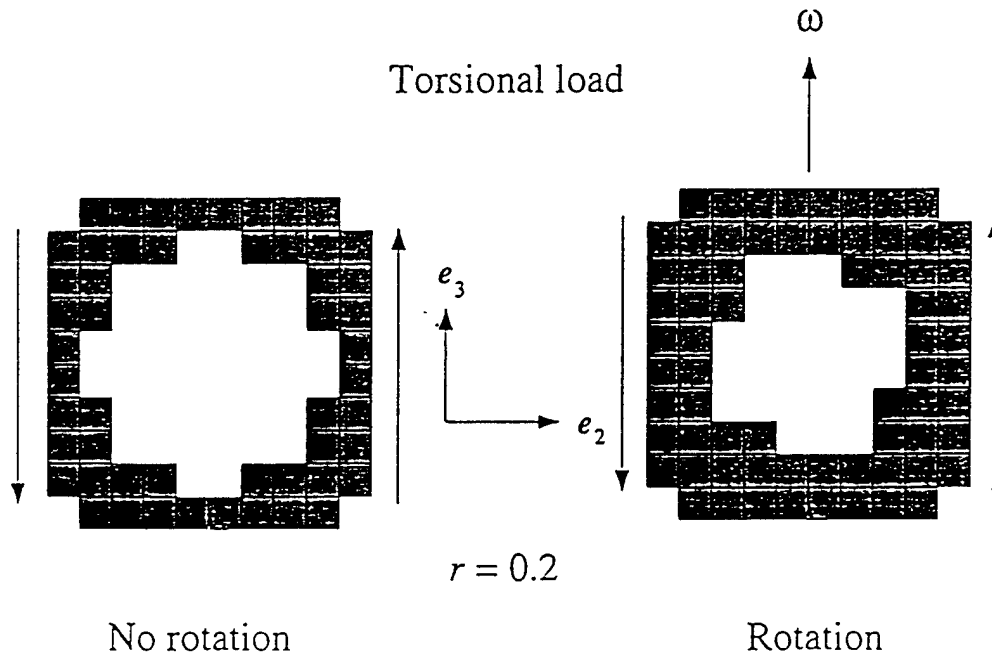
Figure 5: Case 2 (torsional force): cross-sectional view the of optimal design (for \tau = 0.2 ) without a field force (left) and with a field force (right).
