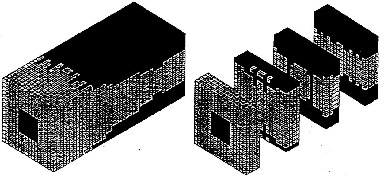
Figure 14- Final topology for E^1/(\max E^2)=1/3 .
