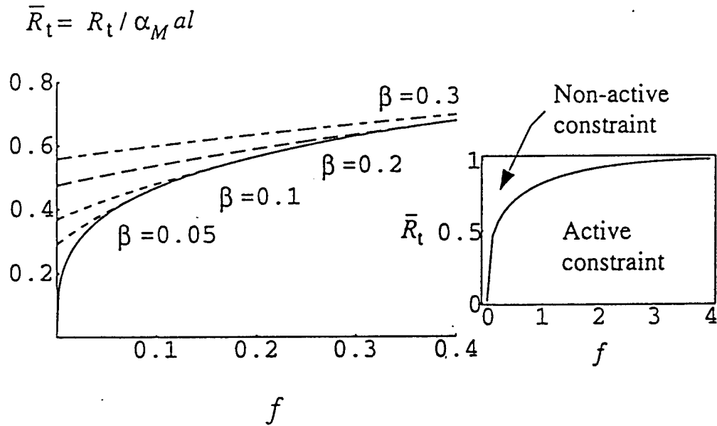
Figure 1: One-dimensional case: normalized total resource \bar{R}_t = R_t / (\alpha_M a l) for different values of the loading and moduli parameters f and \beta . The insert corresponds to the limit case \beta \rightarrow 0 and shows the full range 0 \leq \bar{R}_t \leq 1 . For prescribed values of f and \beta , the resource constraint is not active if the prescribed \bar{R} is above the corresponding \bar{R}_t and active otherwise.
