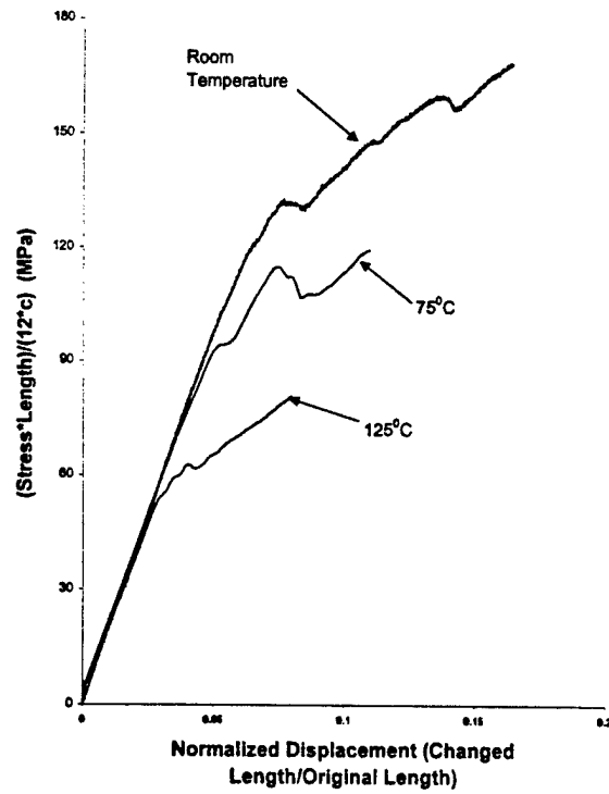
Fig. 29 Effect of Temperature for [0^0_3/+45^0_3/90^0_3/-45^0_3]_{s, type2} (Three Point Bending)
