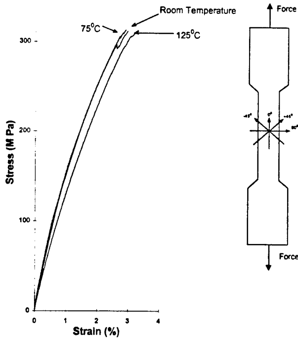
Fig.15 Effect of temperature on [0^{\circ}_3/+45^{\circ}_3/90^{\circ}_3/-45^{\circ}_3]_s specimens
