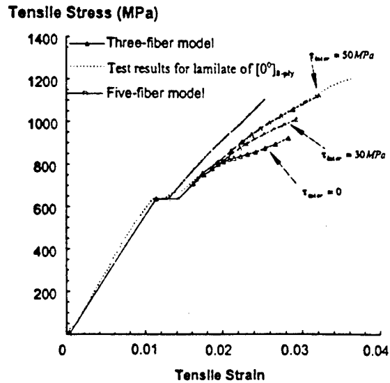
Fig. 2. Comparison between simulated FE and experimental stress-strain curves for S2 glass toughened epoxy ( [0^0]_8-ply )
