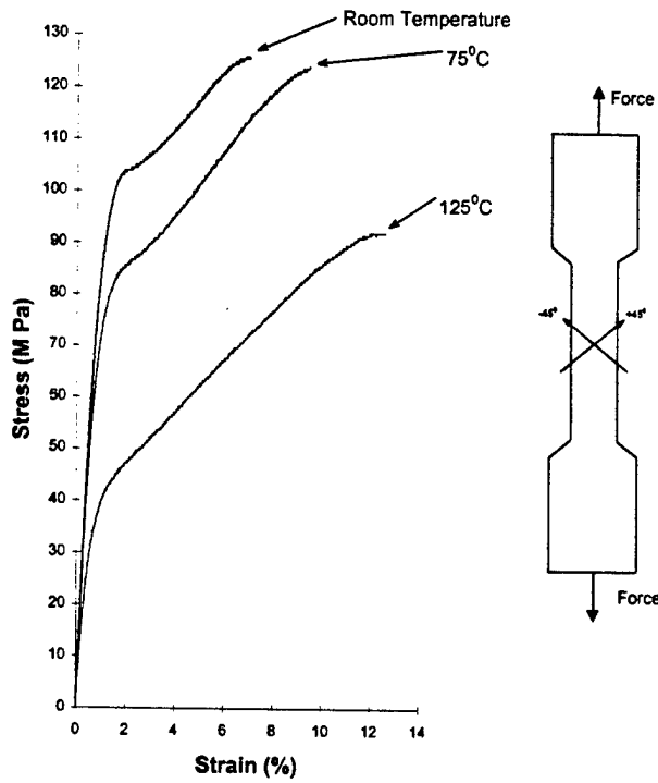
Fig.16 Effect of temperature on [+45^{\circ}/-45^{\circ}]_{3,12s} specimens
