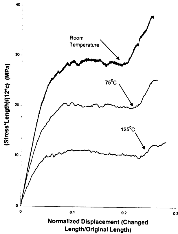
Fig.30 Effect of Temperature for [+45^{\circ}_3/-45^{\circ}_3]_{2s, type2} (Three Point Bending)
