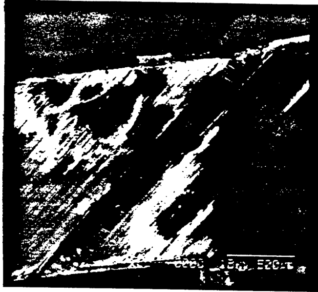
Fig.7 Composites failure at \pm 45^{\circ} (at 80 MPa)
