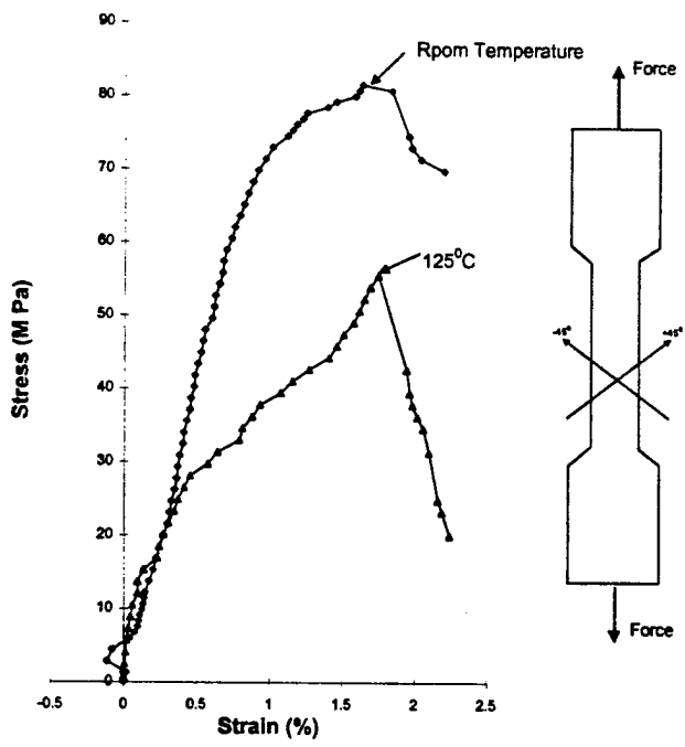
Fig.9 Comparison of room temperature and 125°C results for [+45^0/-45^0/+45^0/-45^0]_s specimens.
