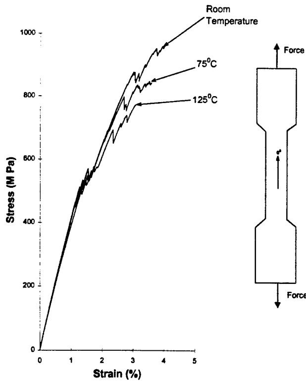
Fig.13 Effect of temperature on [0^\circ]_{24\text{-ply, Type 2}} specimens
