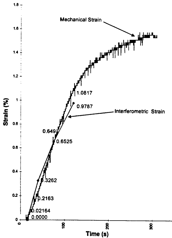
Fig.36 Comparison of the standard MTS results with that of the IDSG for 3 Point Bending measurements on an aluminum sample.
