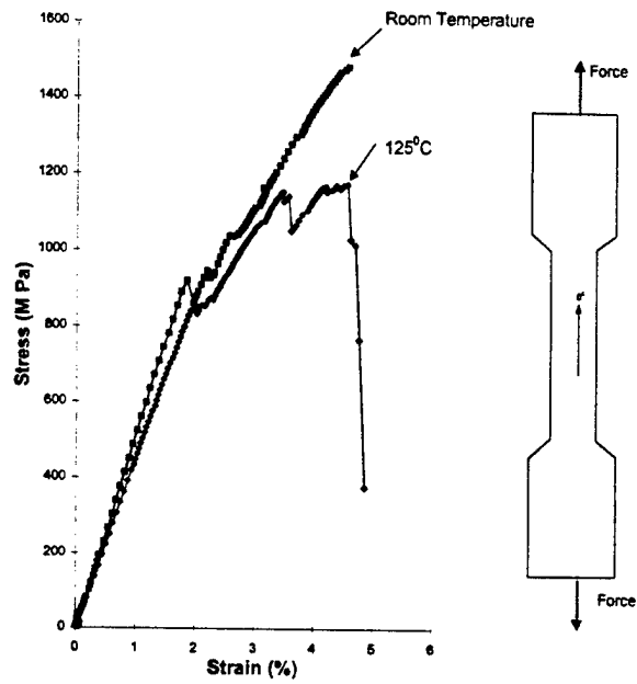
Fig.8 Comparison of room temperature and 125°C results for [0^0]_8 -ply specimens.
