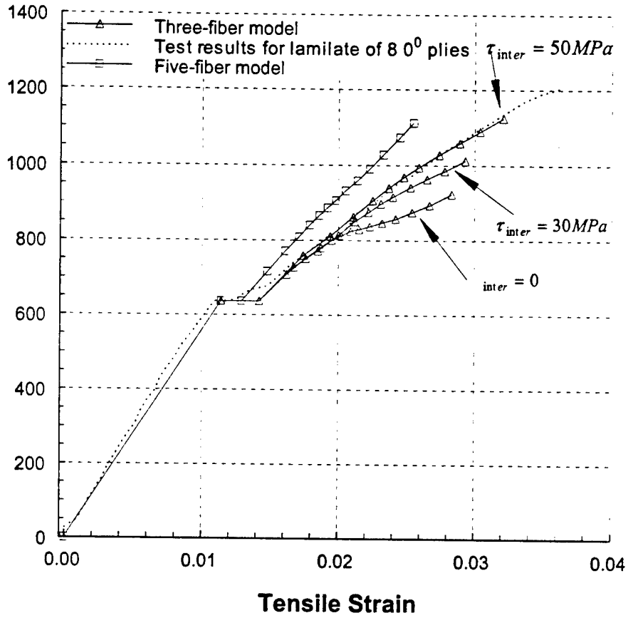
Fig.39 Comparison between simulated FE and experimental stress-strain curves for S2 glass toughened epoxy [0^{\circ}]_{8-ply}
