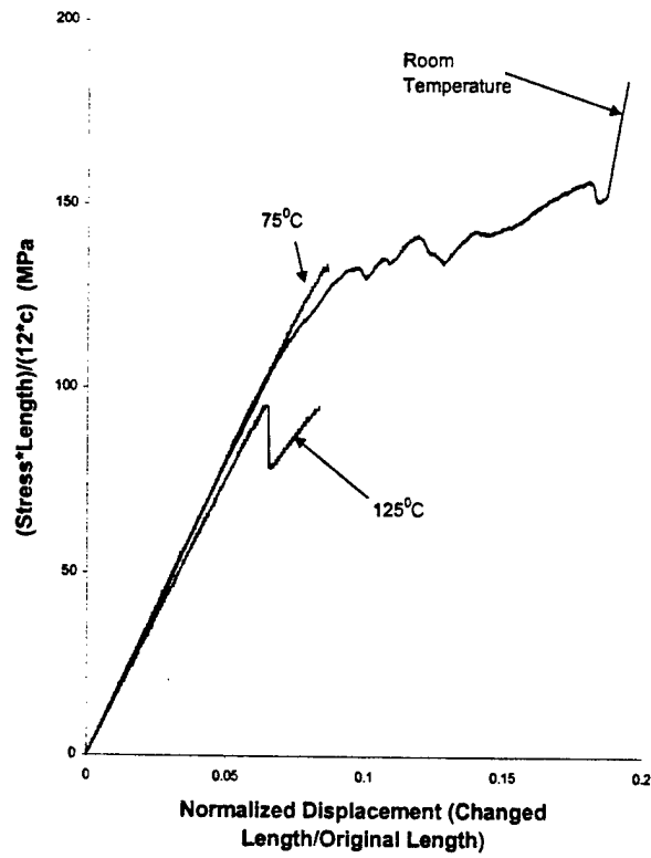
Fig.28 Effect of Temperature for [0^0_3/90^0_3]_{2s, type2} (Three Point Bending)
