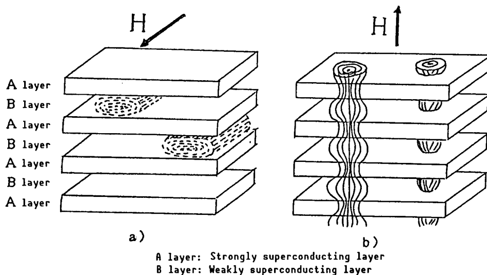
Figure 3. Quantized Magnetic Flux Lines Expected for a Laminated Layer Structure of Two Kinds of Strongly and Weakly Superconducting Layers (a) The intrinsic pinning is not operative. (b) The intrinsic pinning is expected to act in the vertical direction. (The magnetic flux lines are energetically stable when they lie in the weakly superconducting layers.)
