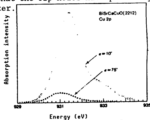
Figure 7(b) Polarized X-Ray Spectra of \text{Cu}2p for a \text{BiSrCaCuO} (2212) Sample (A. Kotani) 5
