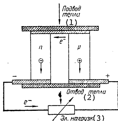
Figure 13. Operating principle of a TELP.
