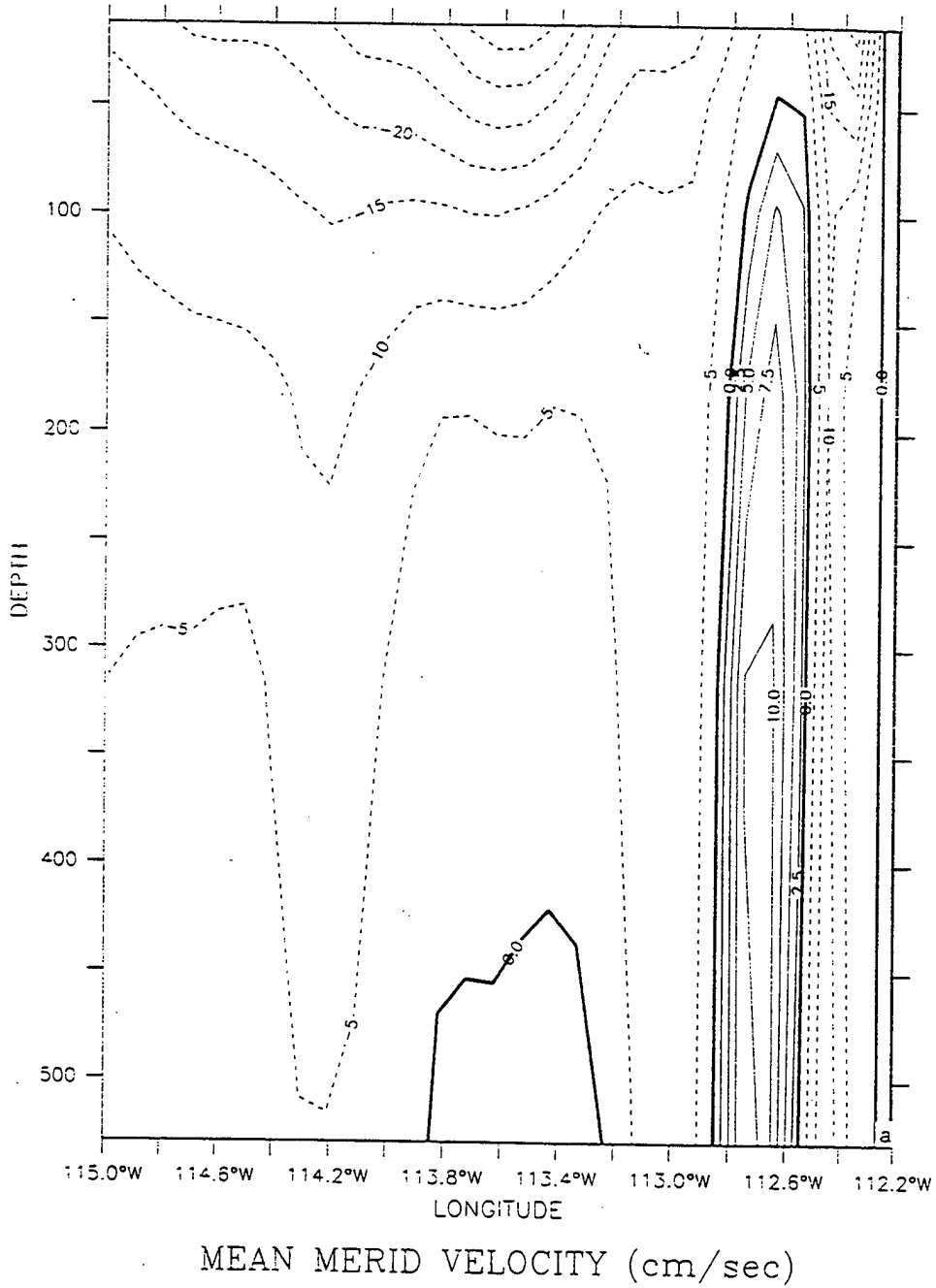
Figure 14. Cross-shore sections of mean v at 25^\circ N (off Cape San Lazaro) for (a) January, (b) April, (c) July, and (d) October of model year 3. The contour interval is 2.5 cm/s (5 cm/s) for poleward (equatorward) flow in (a, b, d) and 5 cm/s for both in (c).
