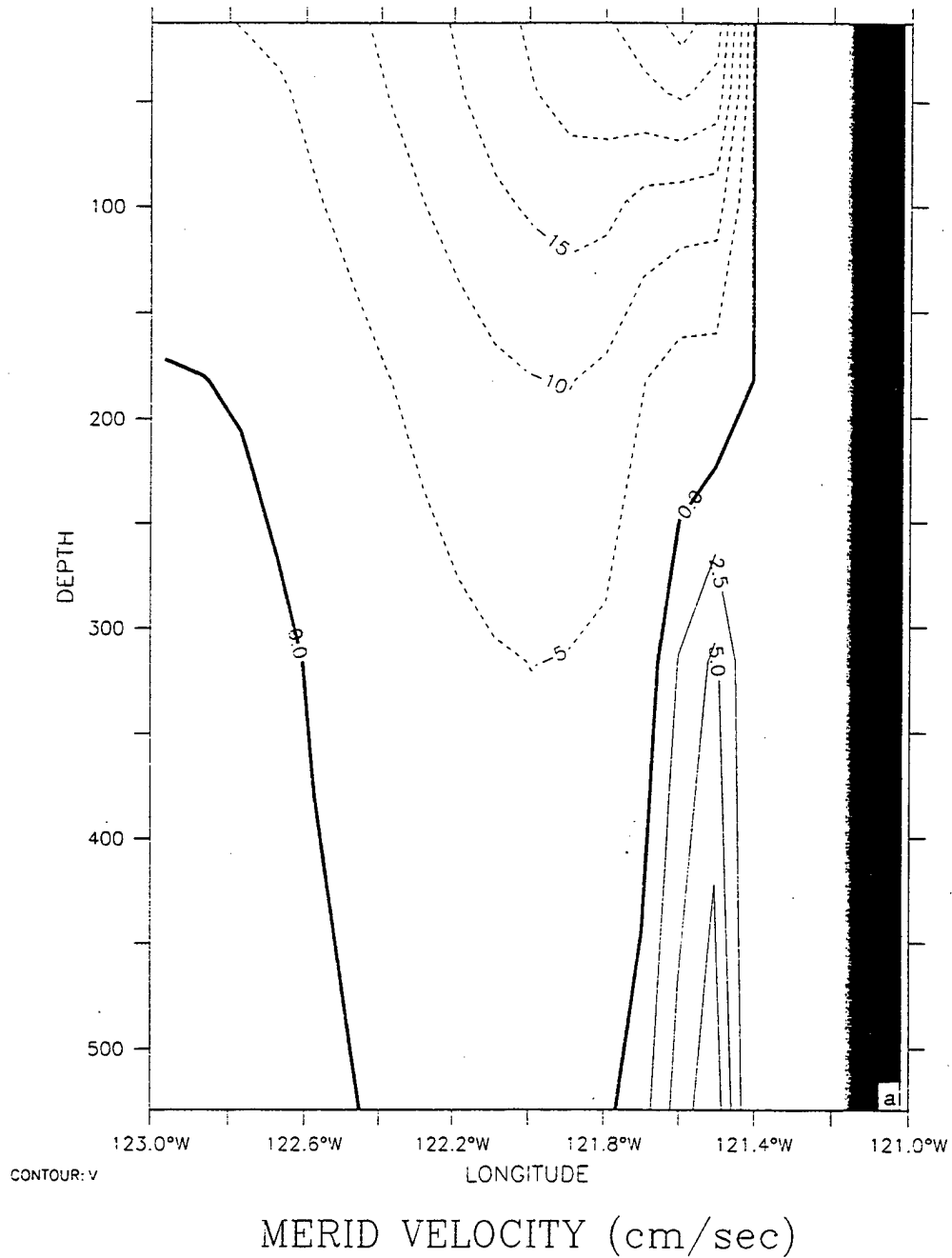
Figure 19. Cross-shore sections of mean v of experiment 2 at 35.7° N in (a) mid-September, (b) mid-October and (c) mid-November. The contour interval is 2.5 cm/s (5 cm/s) for poleward (equatorward) flow.
