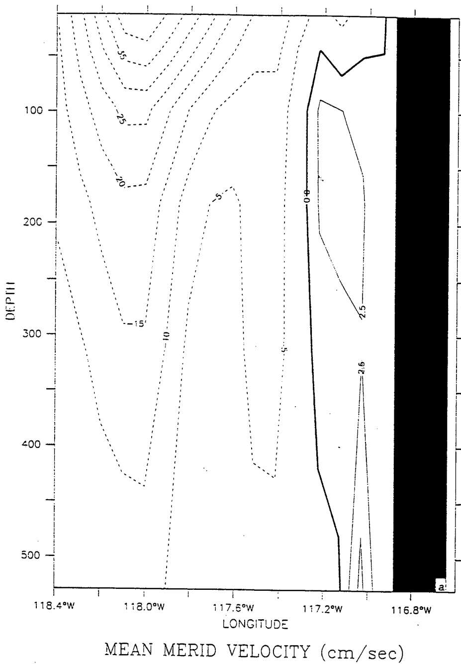
Figure 16. Cross-shore sections of mean v at 32° N for (a) September, (b) October, and (c) November of model year 3. The contour interval is 2.5 cm/s (5 cm/s) for poleward (equatorward) flow.
