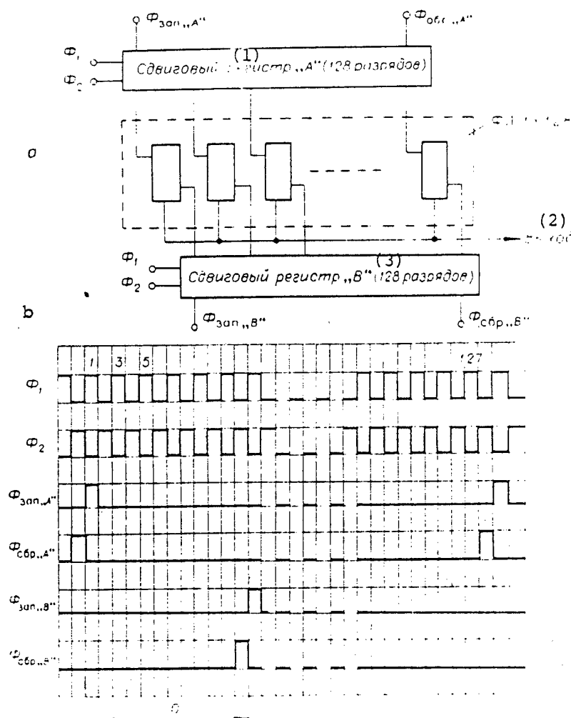
Figure 2. Photodetector (FL) of 128 Light-Sensitive Cells With Two 128-Bit Shift Registers (SR): a--block diagram; b--time diagram required to control shift registers
