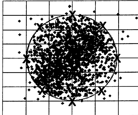
Figure 4. Example distribution of principle components for a specific design task. Eight representative cases from perimeter of accommodation circle are marked.
