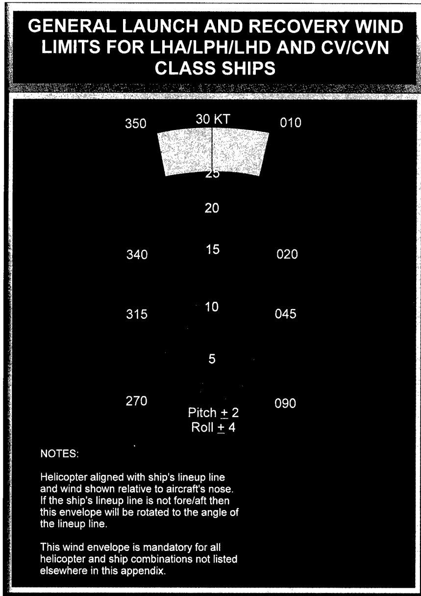
Figure C-2. General Launch and Recovery Wind Limits for LHA/LPH/LHD and CV/CVN Class Ships
