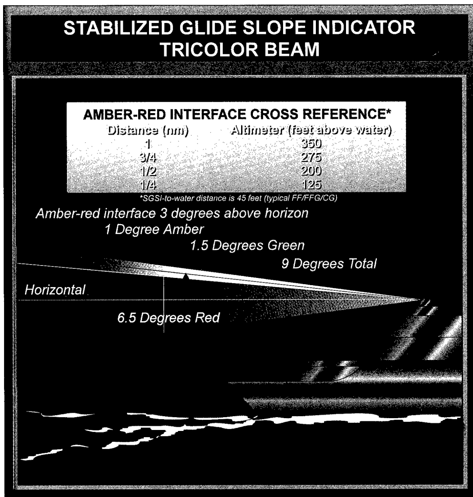
Figure V-3. Stabilized Glide Slope Indicator Tricolor Beam
