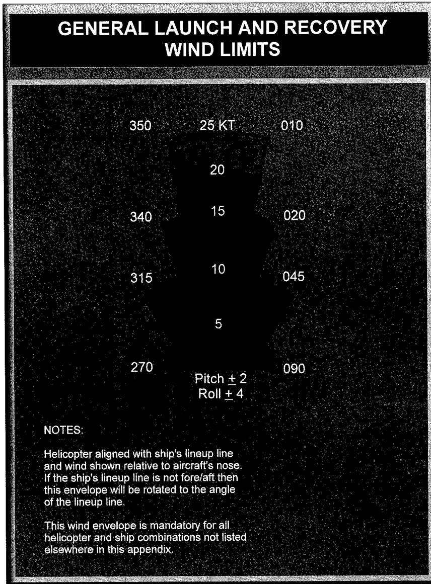
Figure C-1. General Launch and Recovery Wind Limits
