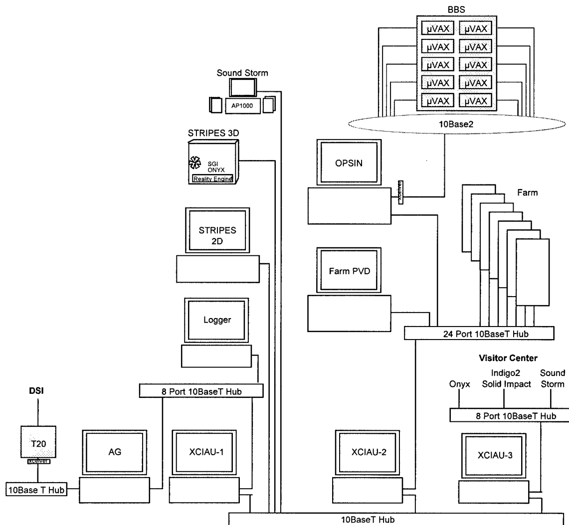
Figure 4.6.1-1 NSC Networks
