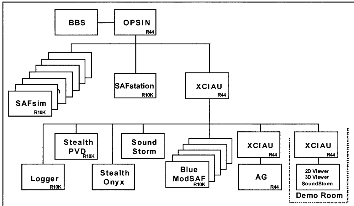
Figure 5.4.2.2-1 NSC System Configuration Diagram, Functional Test 1
