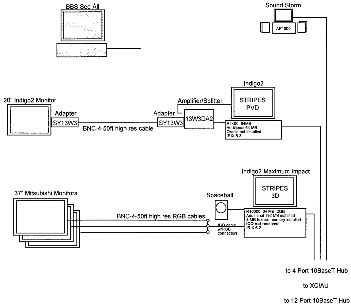
Figure 5.2-4 National Simulation System Diagram, Visitor Center
