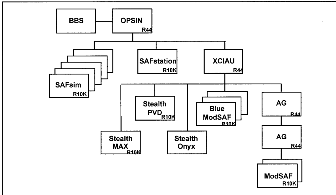
Figure 5.4.1.2-1 OSF System Configuration Diagram, Integration and Test
