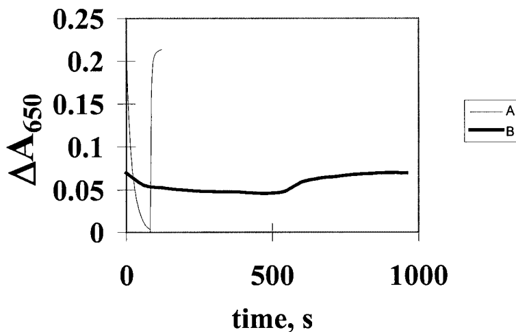
Figure 6. Time-dependent oxidation of [Os II (bpy) 2 (4,4'-(CO 2 H) 2 )] 2+ to Os III on ZrO 2 loaded from CH 3 CN (A) compared to a ZrO 2 surface diluted with [Ru II (bpy) 2 (4,4'-(CO 2 H) 2 )] 2+ (2:1) Ru II :Os II . The potential of the underlying ITO electrode was stepped to 1.3 V vs. Ag/AgNO 3 and then to 0 V. Absorbance-time changes were monitored at 650 nm.
