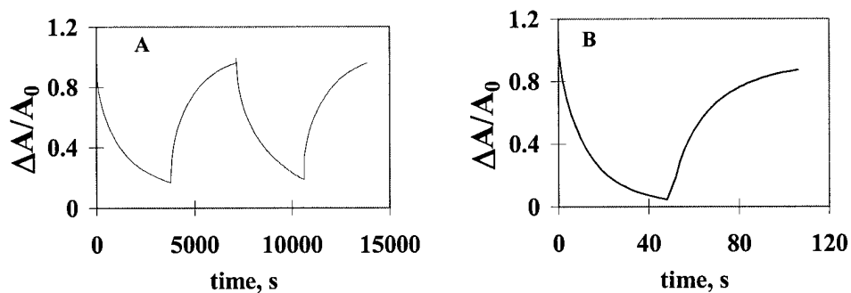
Figure 4 Time-dependent oxidation of [\text{Os}^{\text{II}}(\text{bpy})_2(4,4'-(\text{CO}_2\text{H})_2)]^{2+} to \text{Os}^{\text{III}} on \text{TiO}_2 loaded from EtOH (A) compared to \text{CH}_3\text{CN} (B). The potential of the underlying ITO electrode was stepped to 1.3 V vs. \text{Ag}/\text{AgNO}_3 and absorption-time changes monitored at 650 nm.
