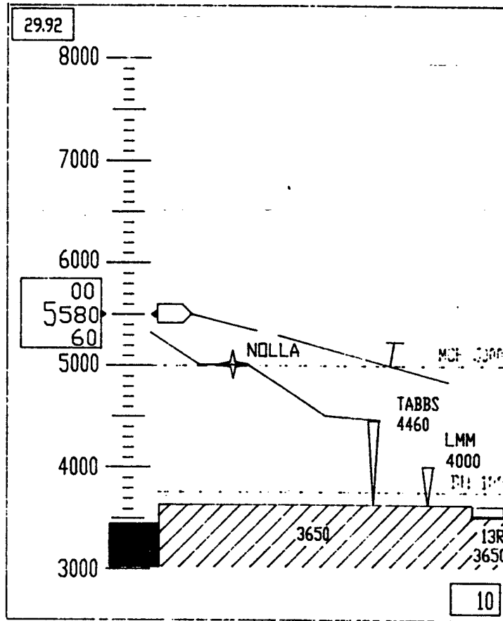
Figure 3.- Vertical situation display.
