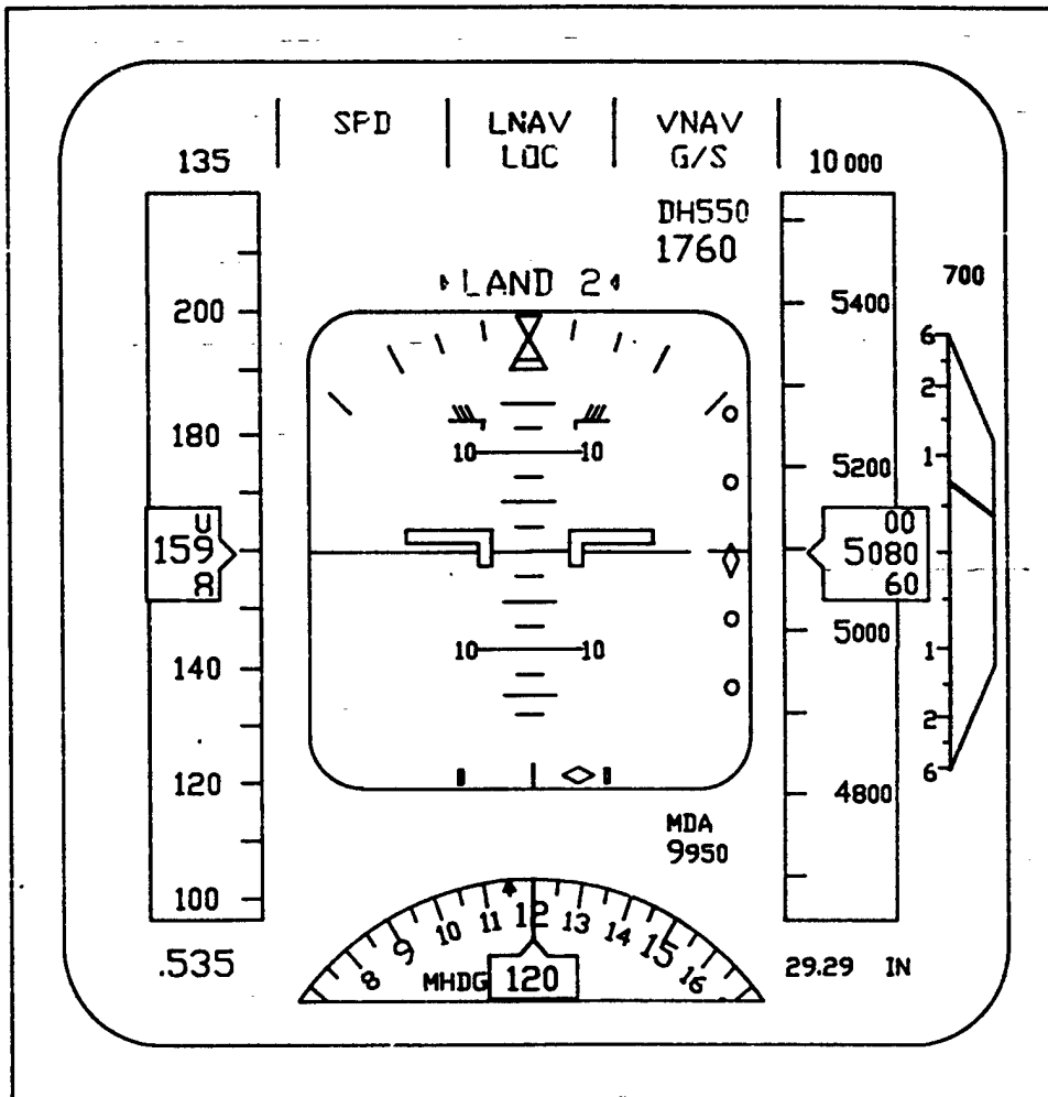
Figure 1.- Primary flight display.
