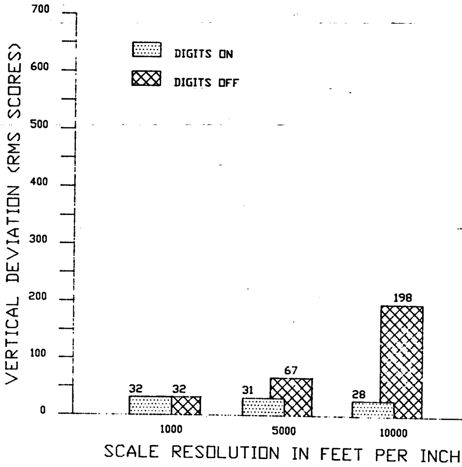
Figure 6.- Level-off segment (graphics on) means for digits x resolution.
