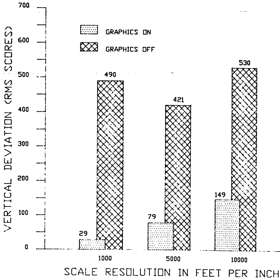
Figure 4.- Overall means for graphics x resolution.
